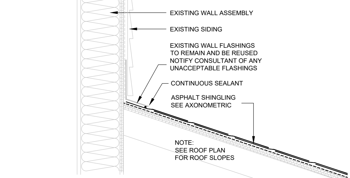
1 1/2" = 1'-0" D1 TYPICAL ROOF/WALL TRANSITION DETAIL A-301
