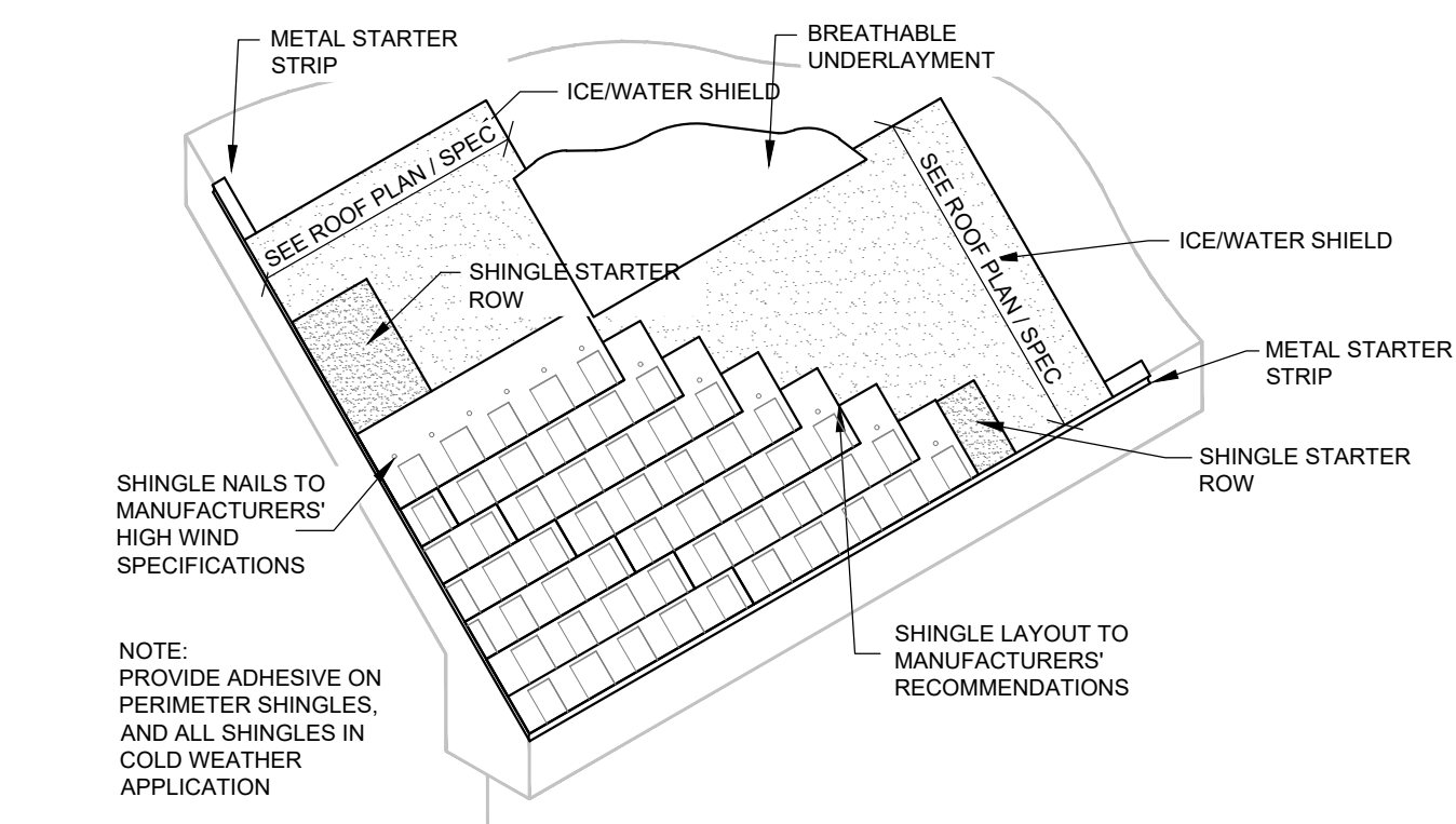
1 1/2" = 1'-0" D4 TYPICAL SHINGLING AXONOMETRIC A-301
