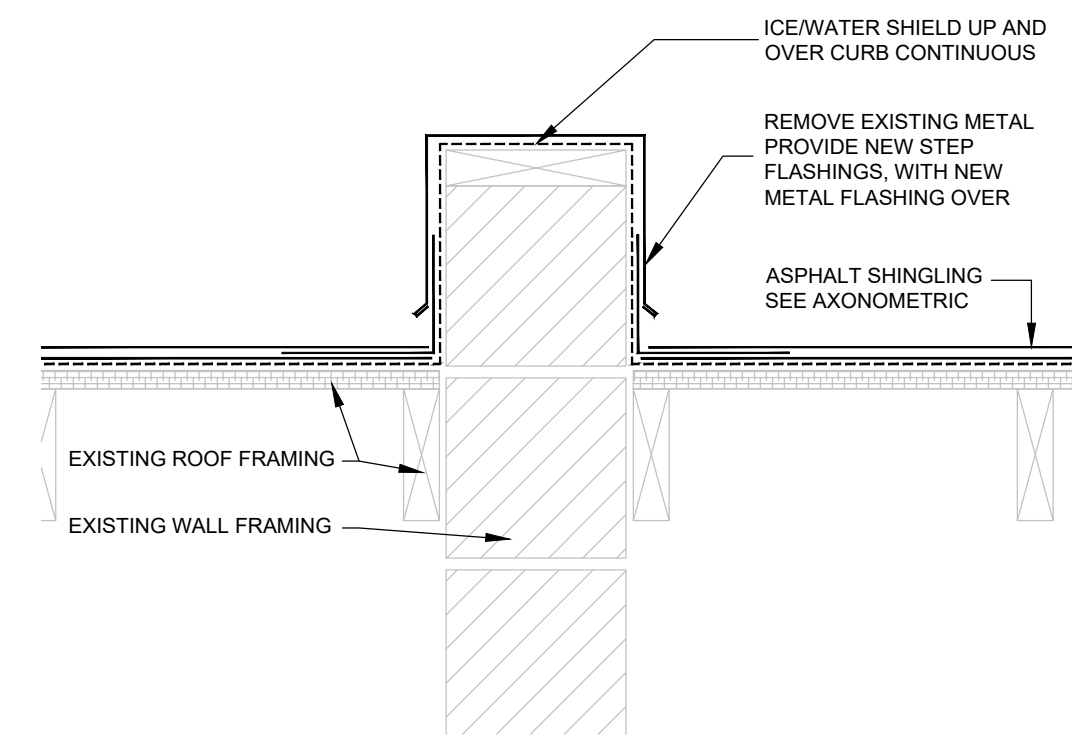
1 1/2" = 1'-0" C2 TYPICAL CURB DETAIL A-301
