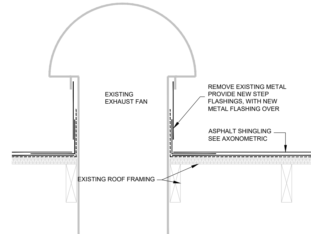
1 1/2" = 1'-0" D2 TYPICAL CURB DETAIL A-301
