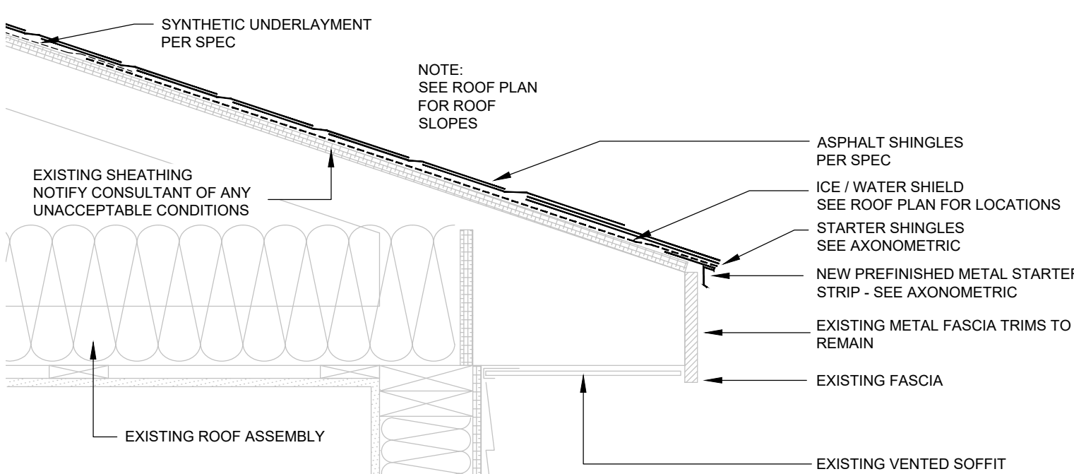
1 1/2" = 1'-0" C1 TYPICAL EAVE DETAIL A-301
