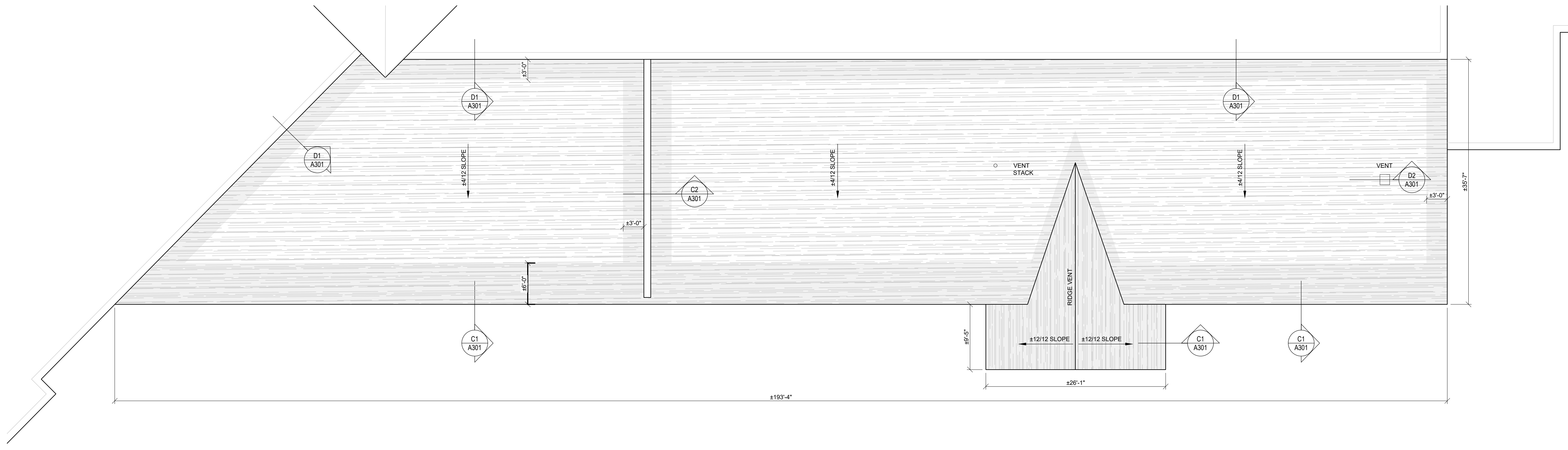
1/8" = 1'-0" A1 ROOF PLAN A-301
