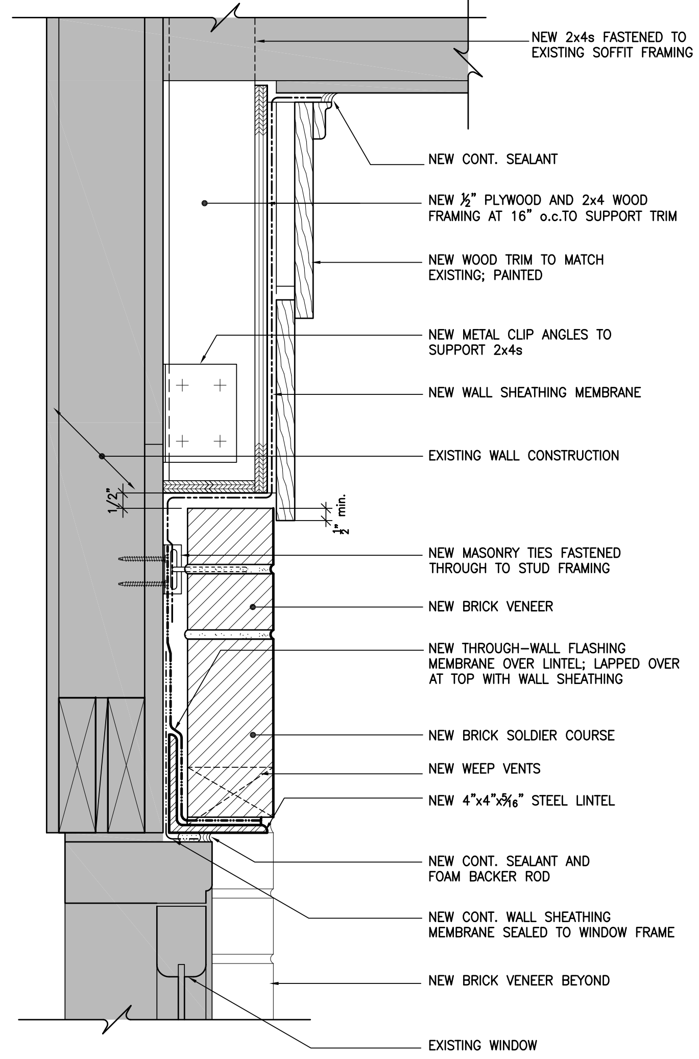
4 A-1 SECTION DETAIL WINDOW HEAD SCALE: 3" = 1'-0"
