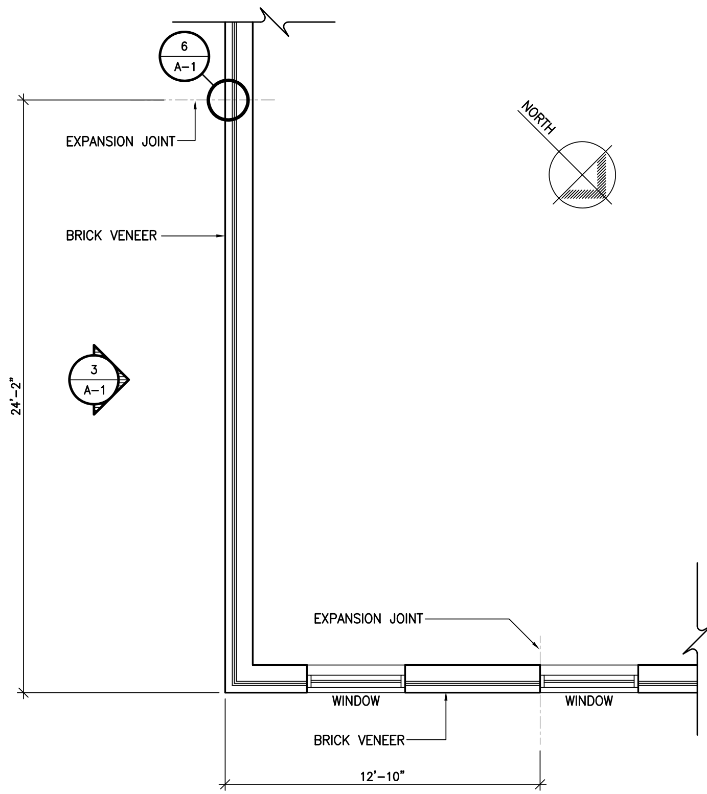
1 A-1 PARTIAL PLAN SCALE: 1/4" = 1'-0"
