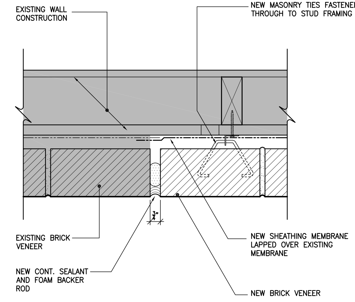
6 A-1 PLAN DETAIL EXPANSION JOINT SCALE: 3" = 1'-0"
