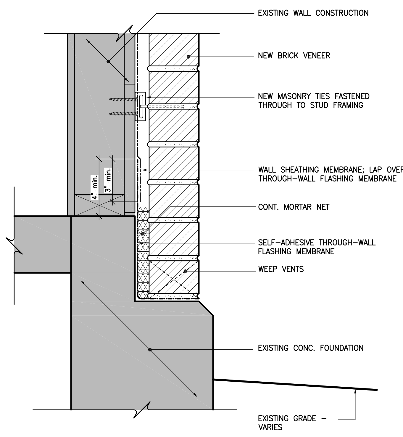
5 A-1 SECTION DETAIL BASE OF WALL SCALE: 3" = 1'-0"
