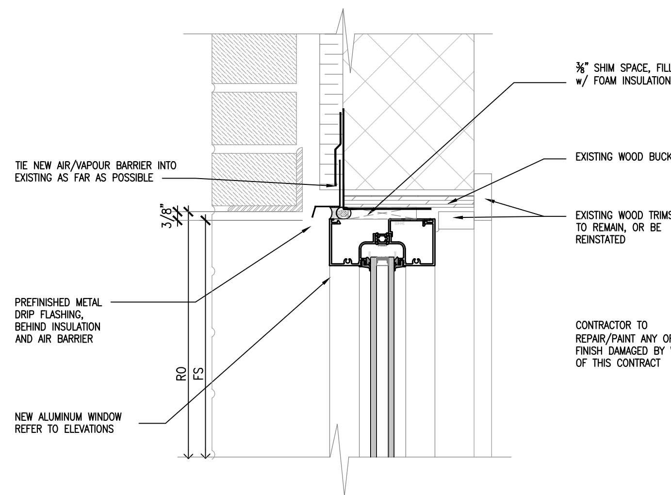
3"=1'-0" C2 SECTION - WINDOW HEAD A-301
