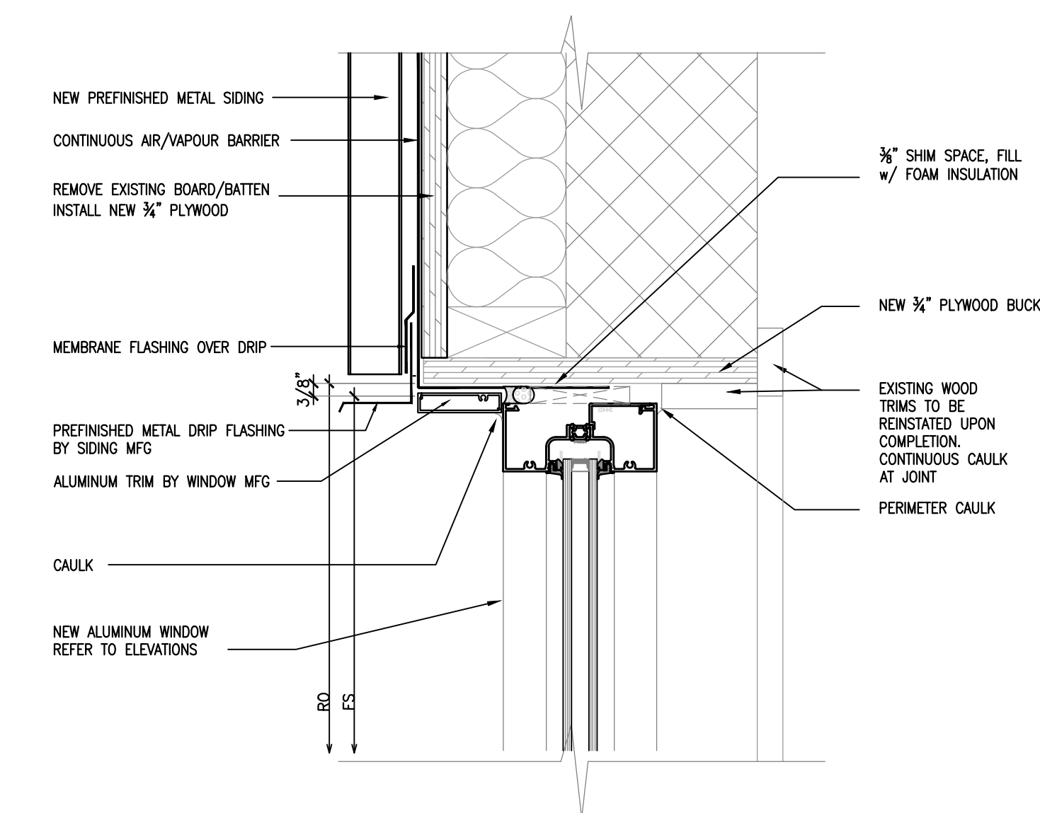
3"=1'-0" D3 SECTION - WINDOW HEAD A-301
