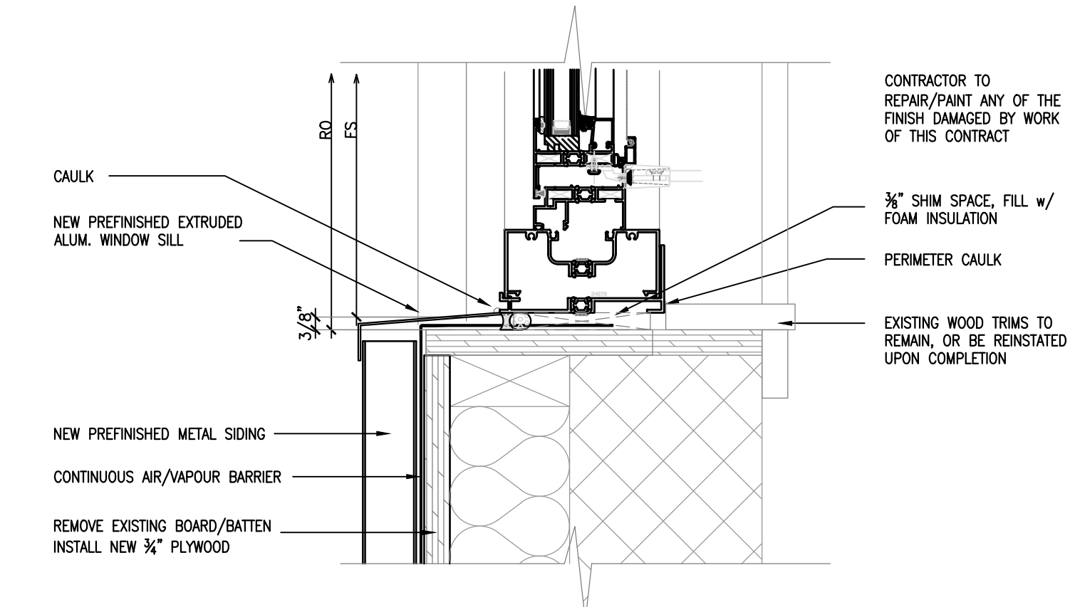
3"=1'-0" C3 SECTION - WINDOW SILL A-301
