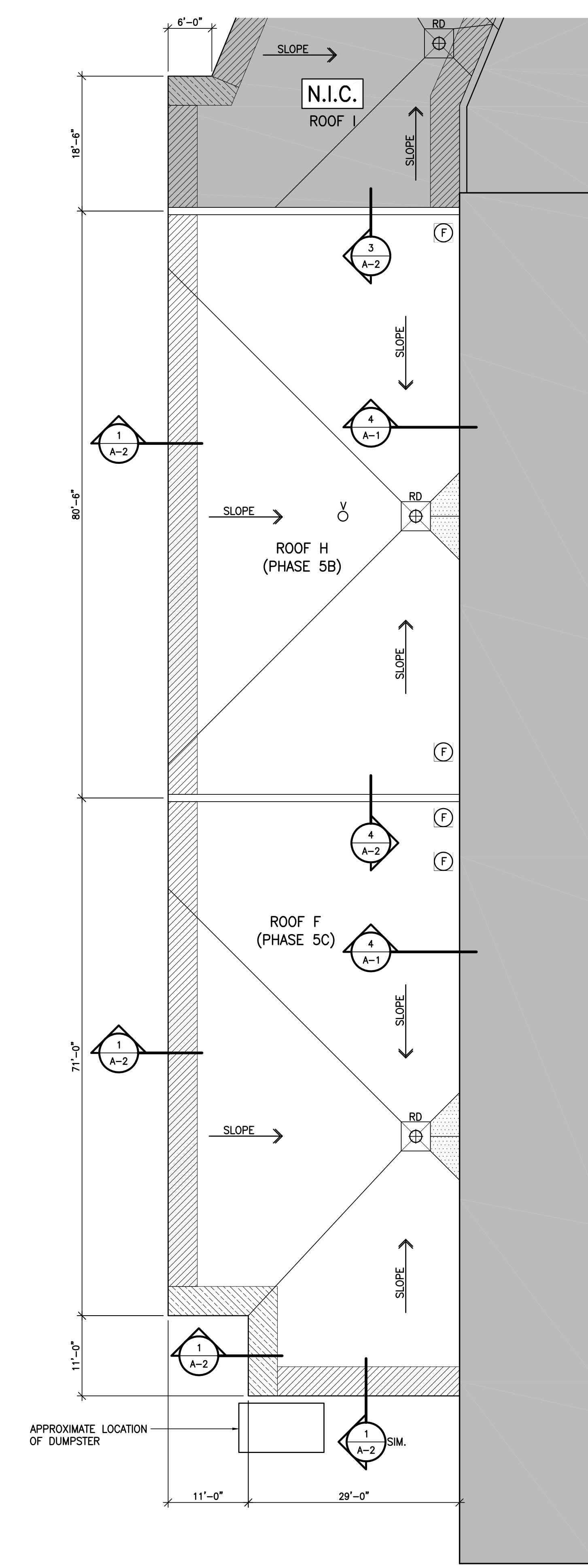
3 PLAN - ROOF 'H' AND 'F' A-1 SCALE: 3/32" = 1'-0"
