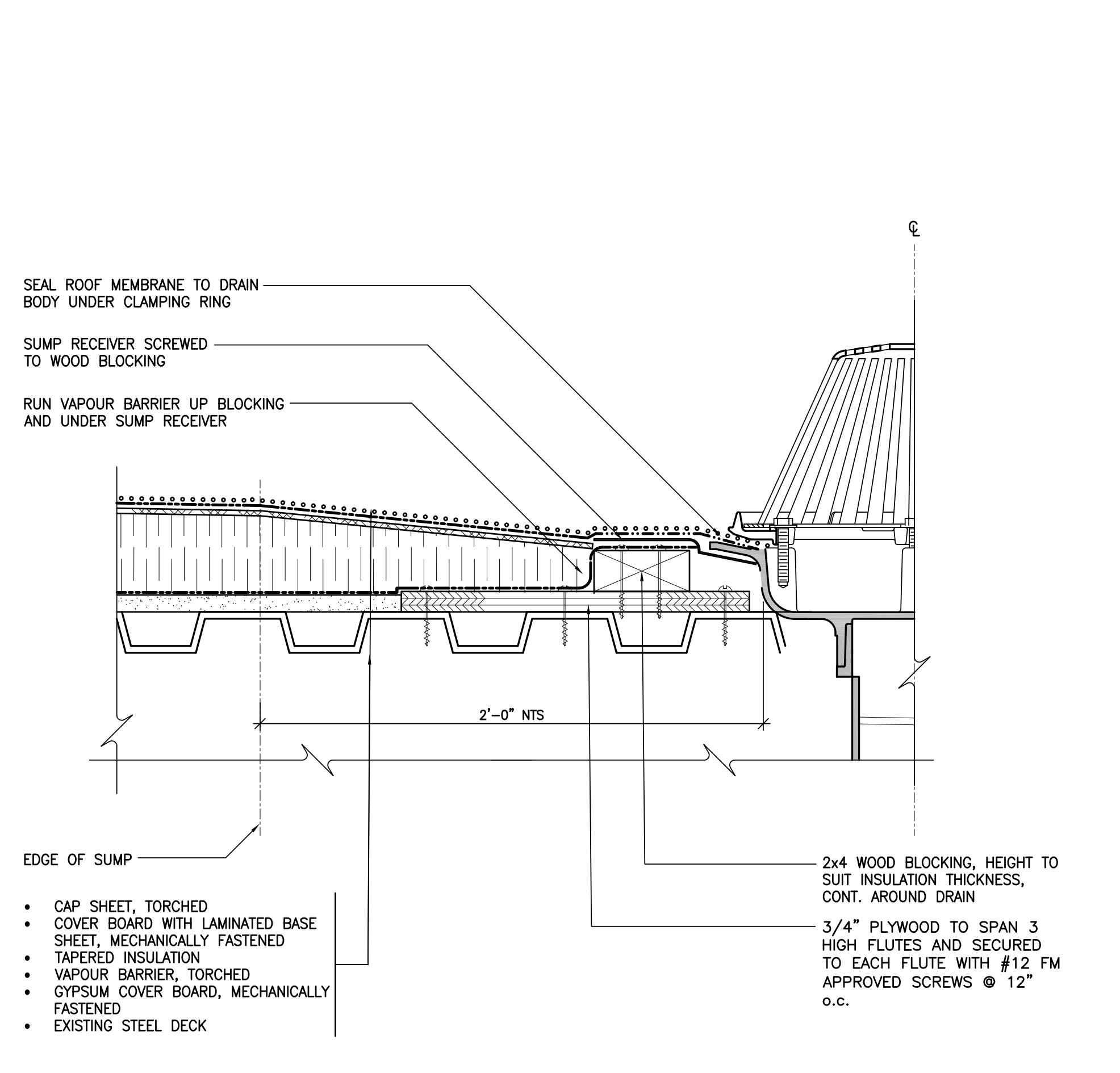
6 SECTION DETAIL ROOF DRAIN
