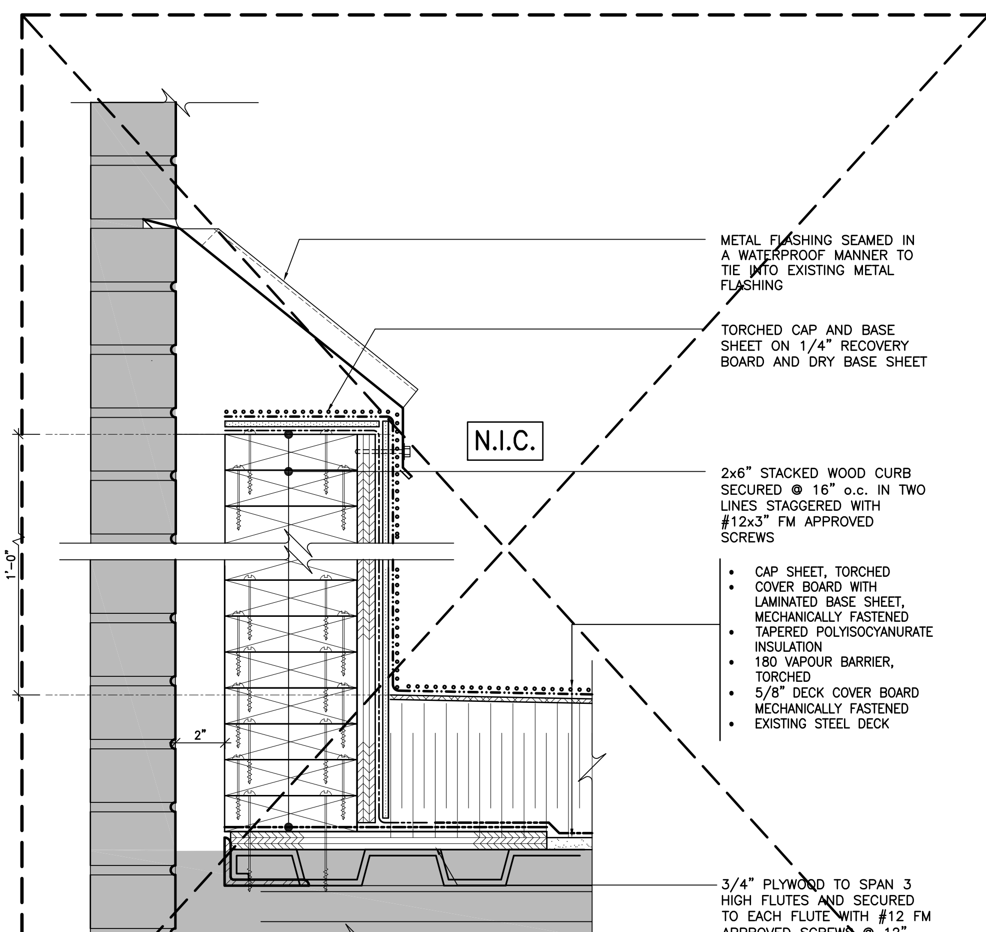
5 SECTION DETAIL CHIMNEY CURB N.I.C.
