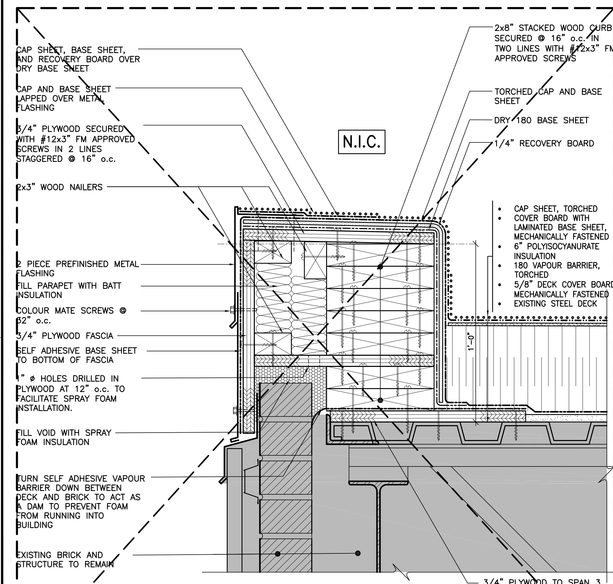
2 SECTION DETAIL ROOF EDGE AT METAL CLADDING N.I.C.
