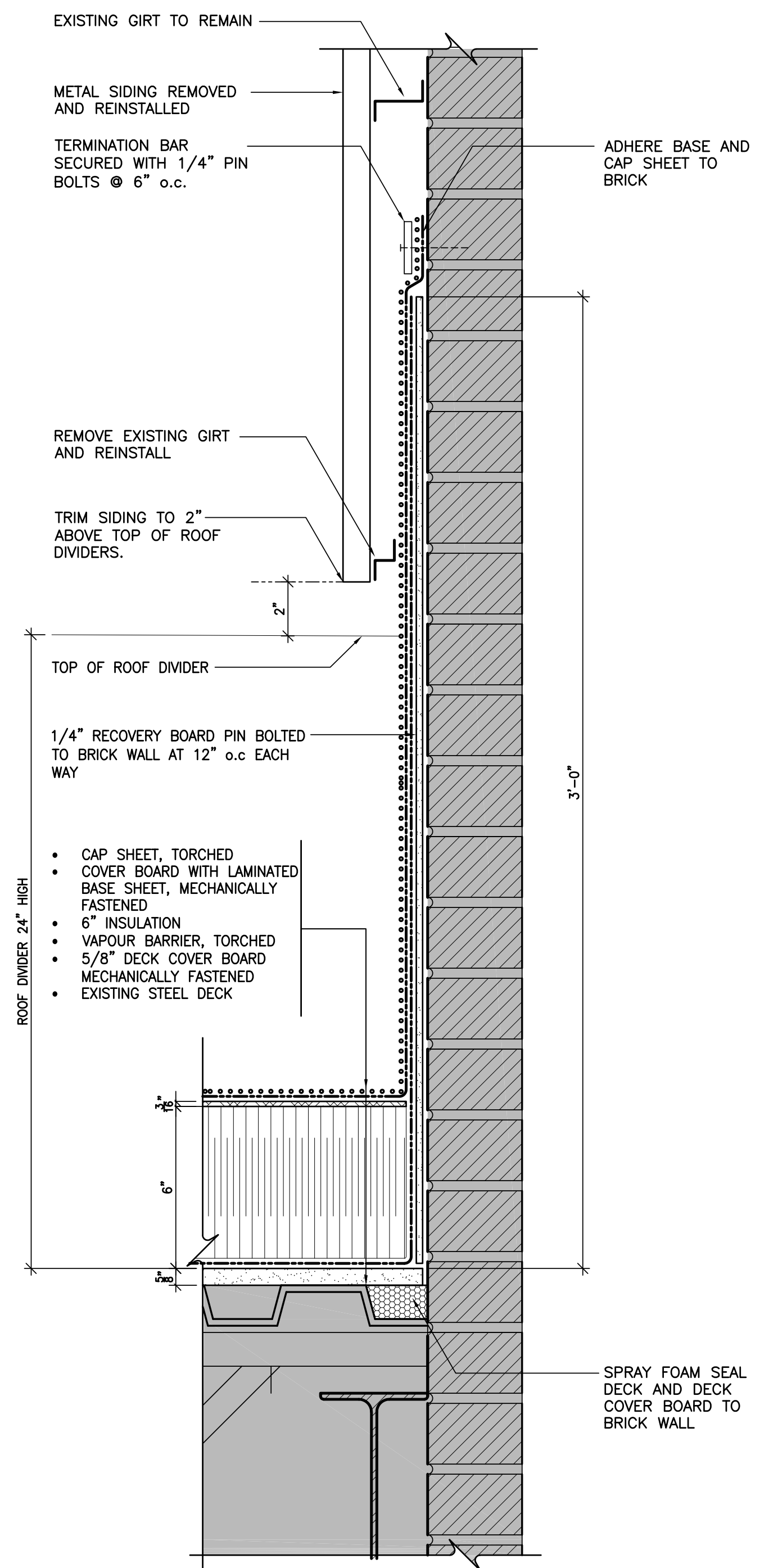
4 SECTION DETAIL METAL CLADDING AT ROOF H AND F A-1 SCALE: 3" = 1'-0"
