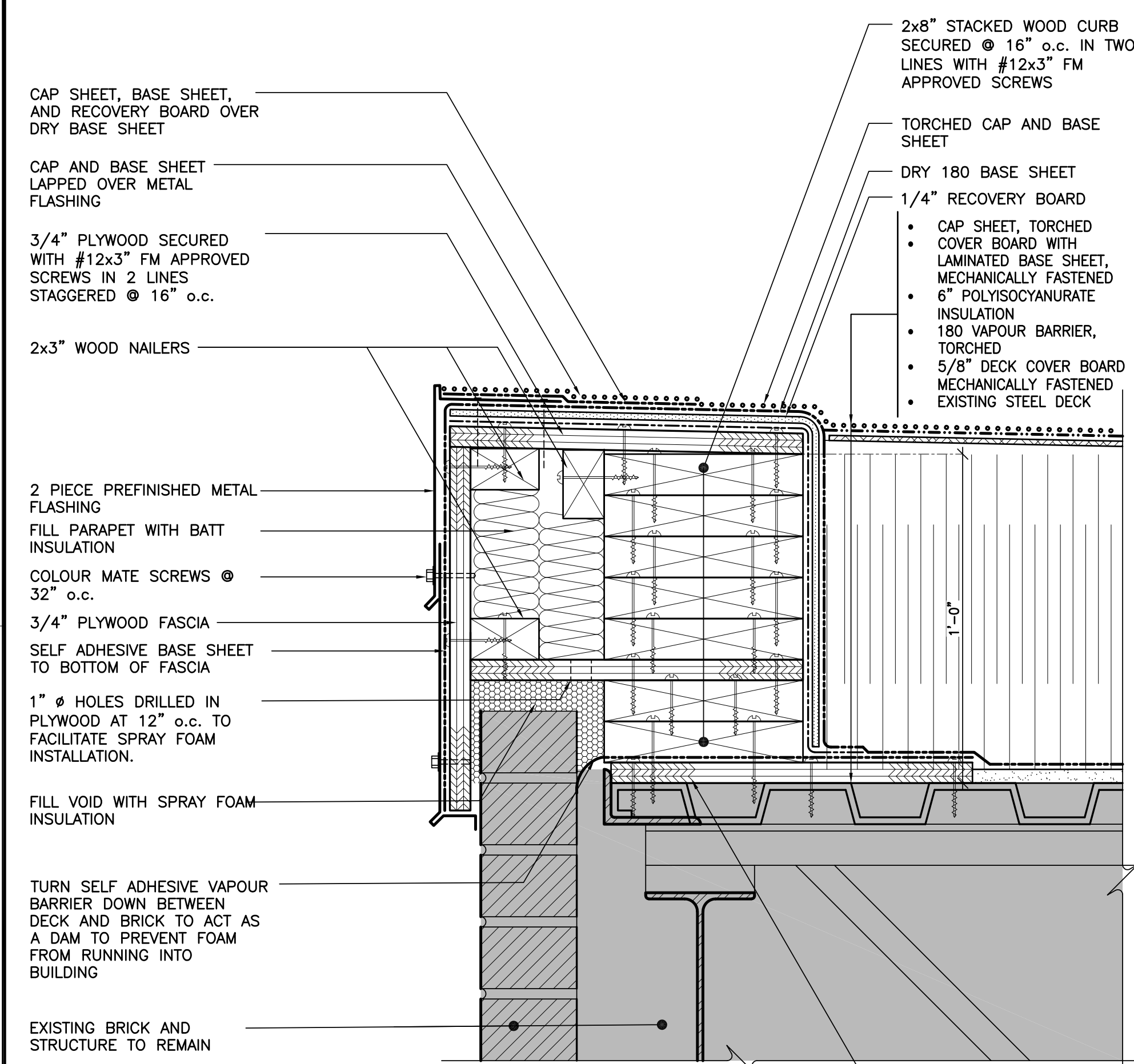
1 SECTION DETAIL ROOF EDGE AT BRICK
