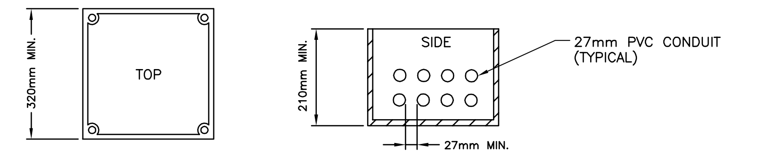
PVC JUNCTION BOX DETAIL (TYPICAL) SCALE: N.T.S.
