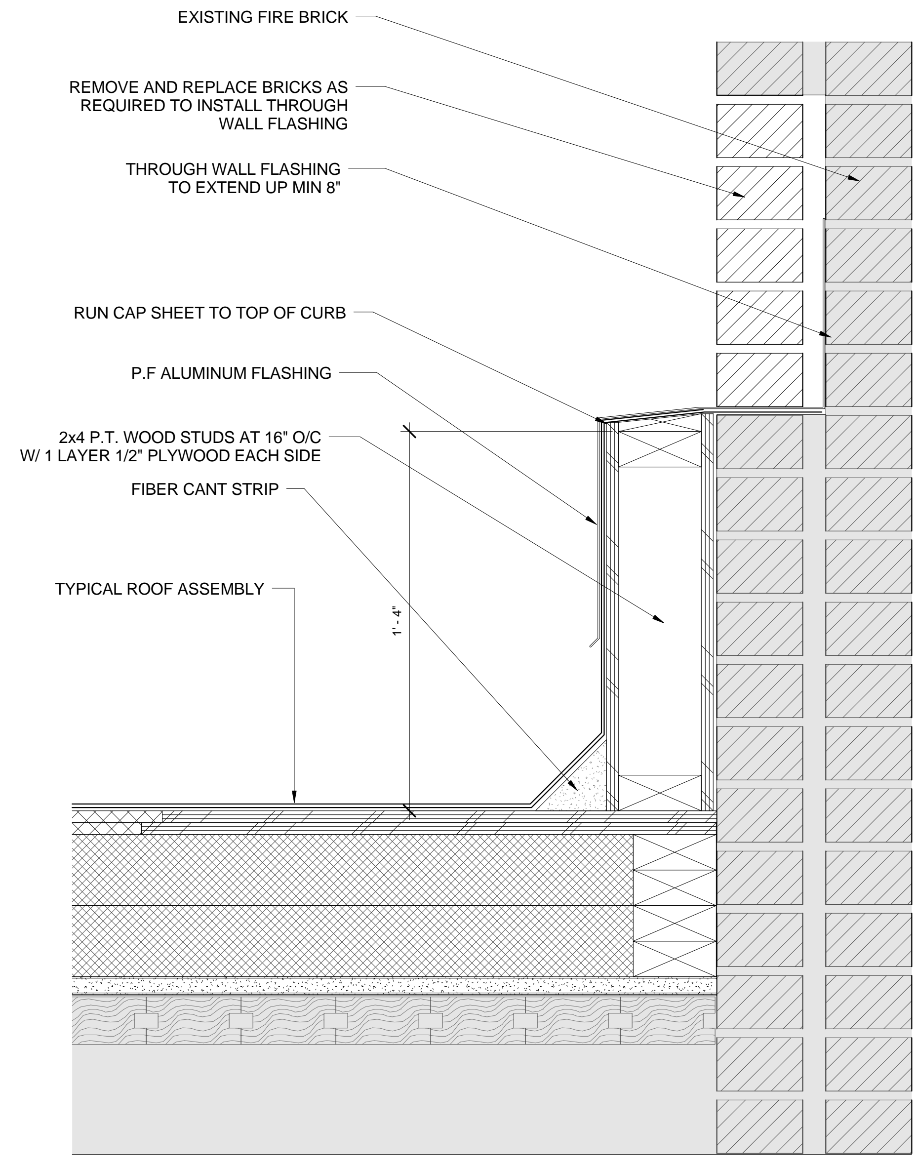
4 DETAIL AT CHIMNEY 3" = 1'-0"
