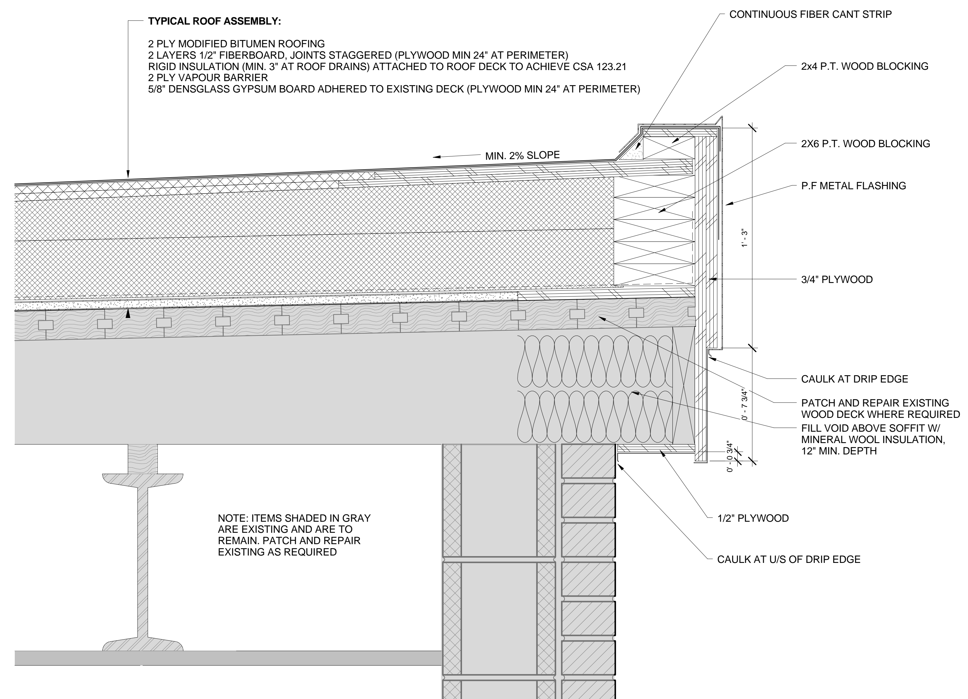
2 PARAPET DETAIL 3" = 1'-0"
