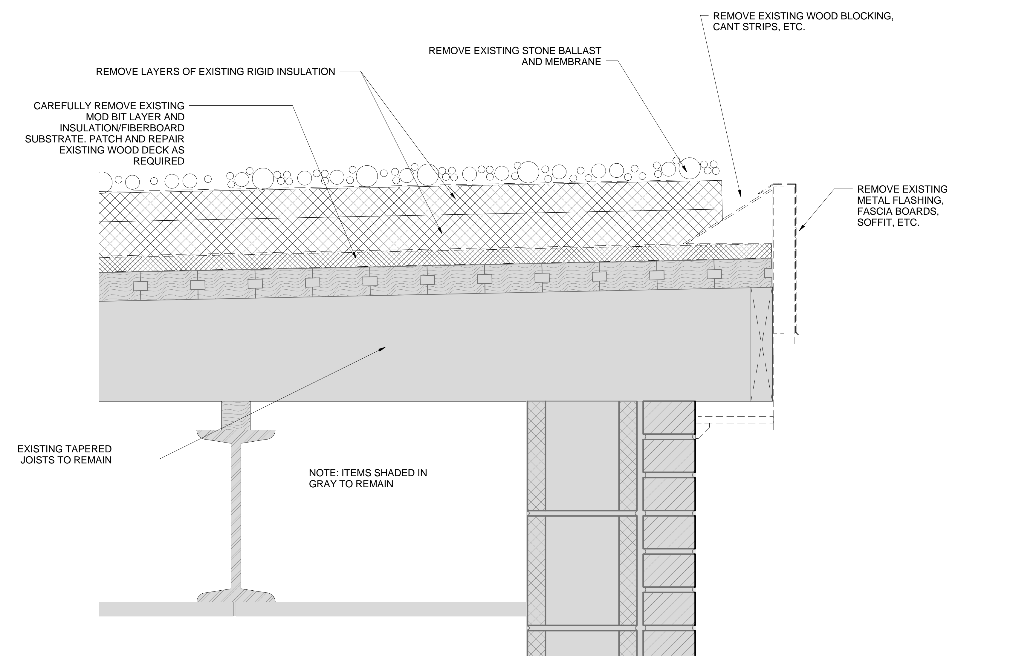
3 PARAPET DETAIL DEMOLITION 3" = 1'-0"
