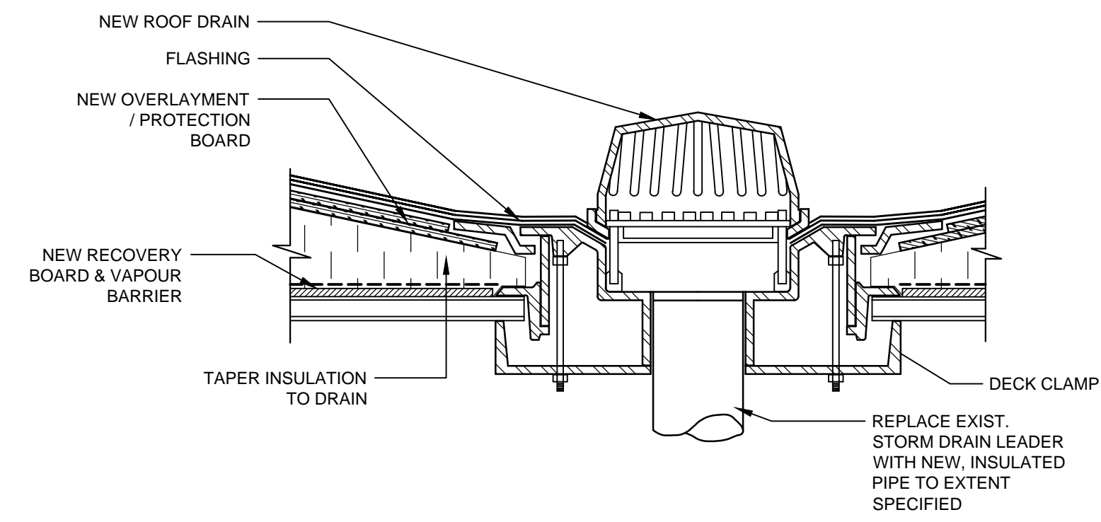
6 ROOF DRAIN DETAIL A-101 1-1/2"-1'-0"
