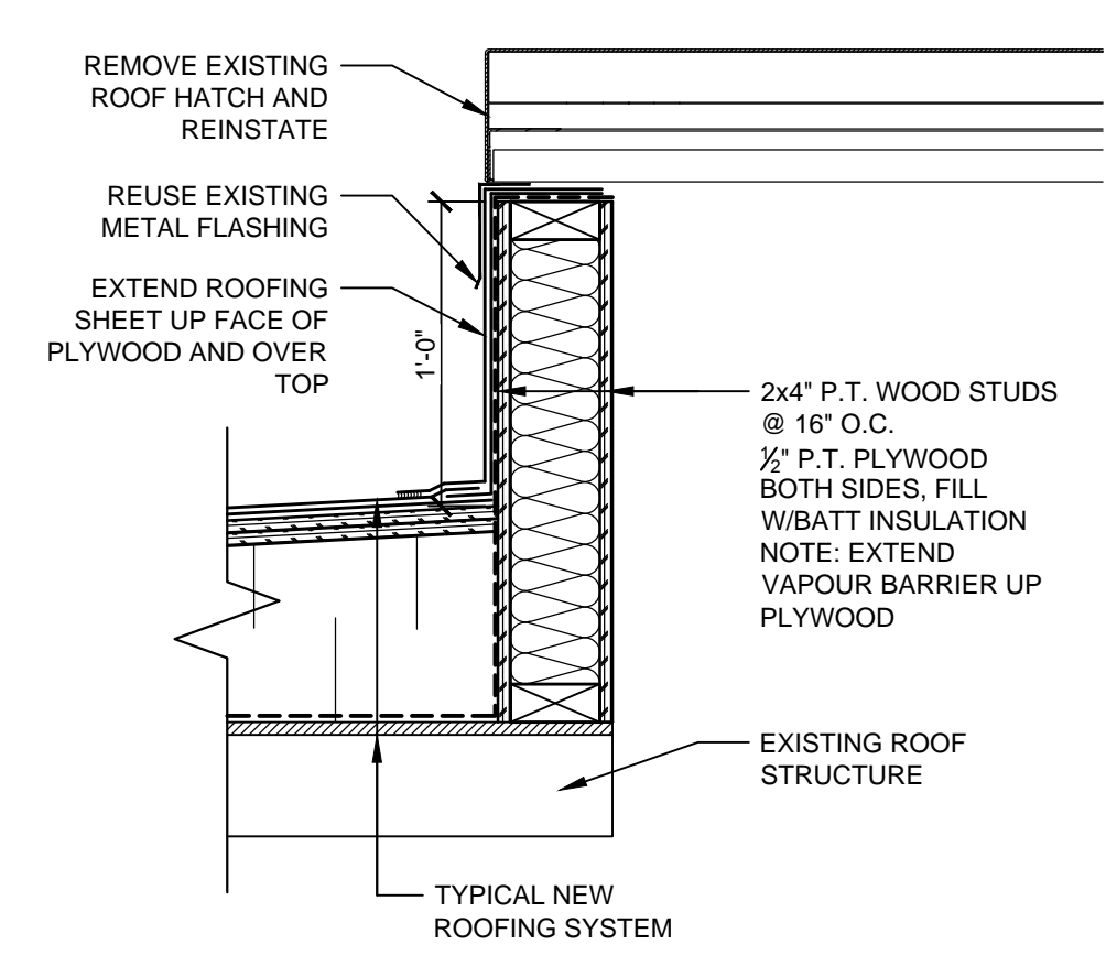
3 ROOF HATCH DETAIL A-101 1-1/2"-1'-0"
