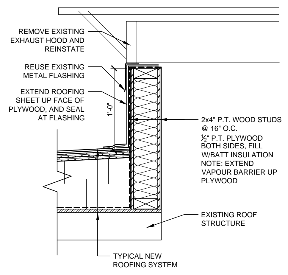
4 EXHAUST HOOD DETAIL A-101 1-1/2"-1'-0"
