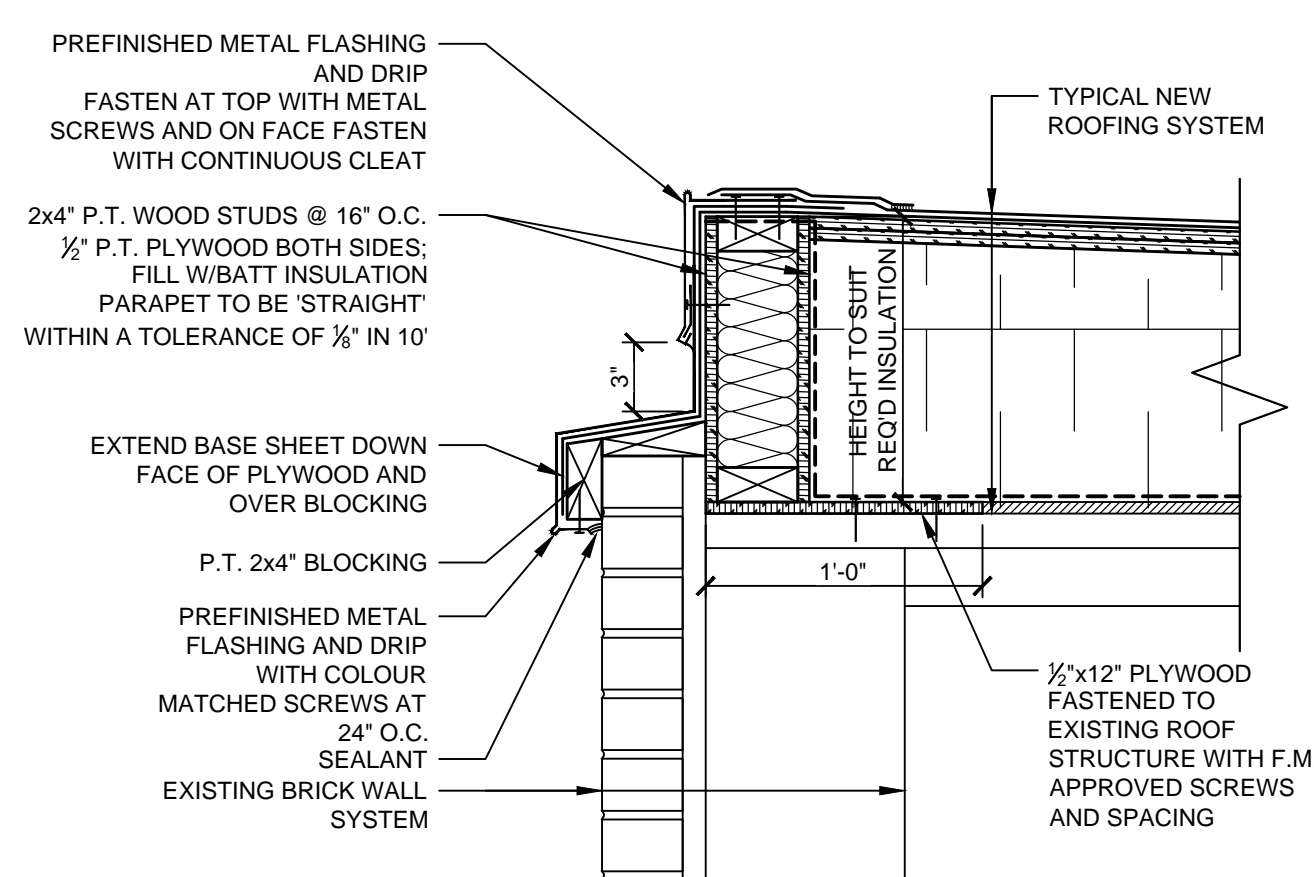
2 PARAPET DETAIL A-101 1-1/2"-1'-0"
