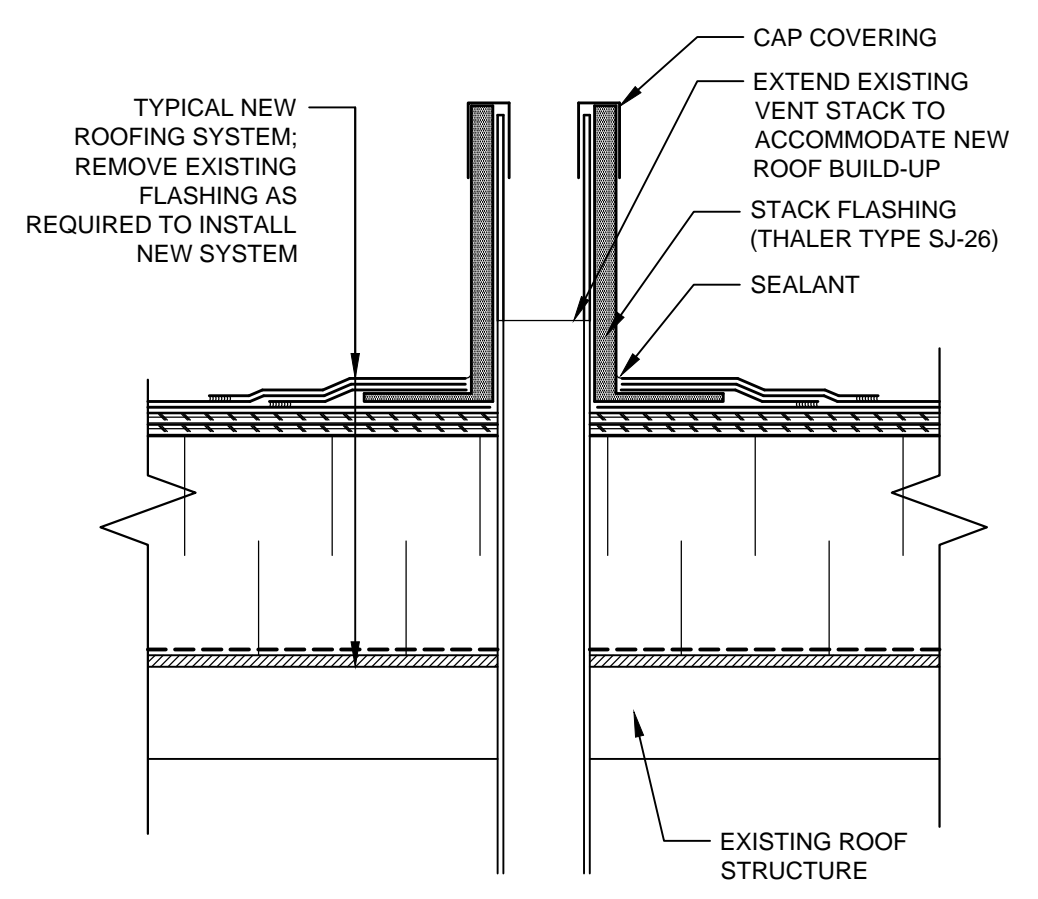
5 VENT STACK DETAIL A-101 1-1/2"-1'-0"
