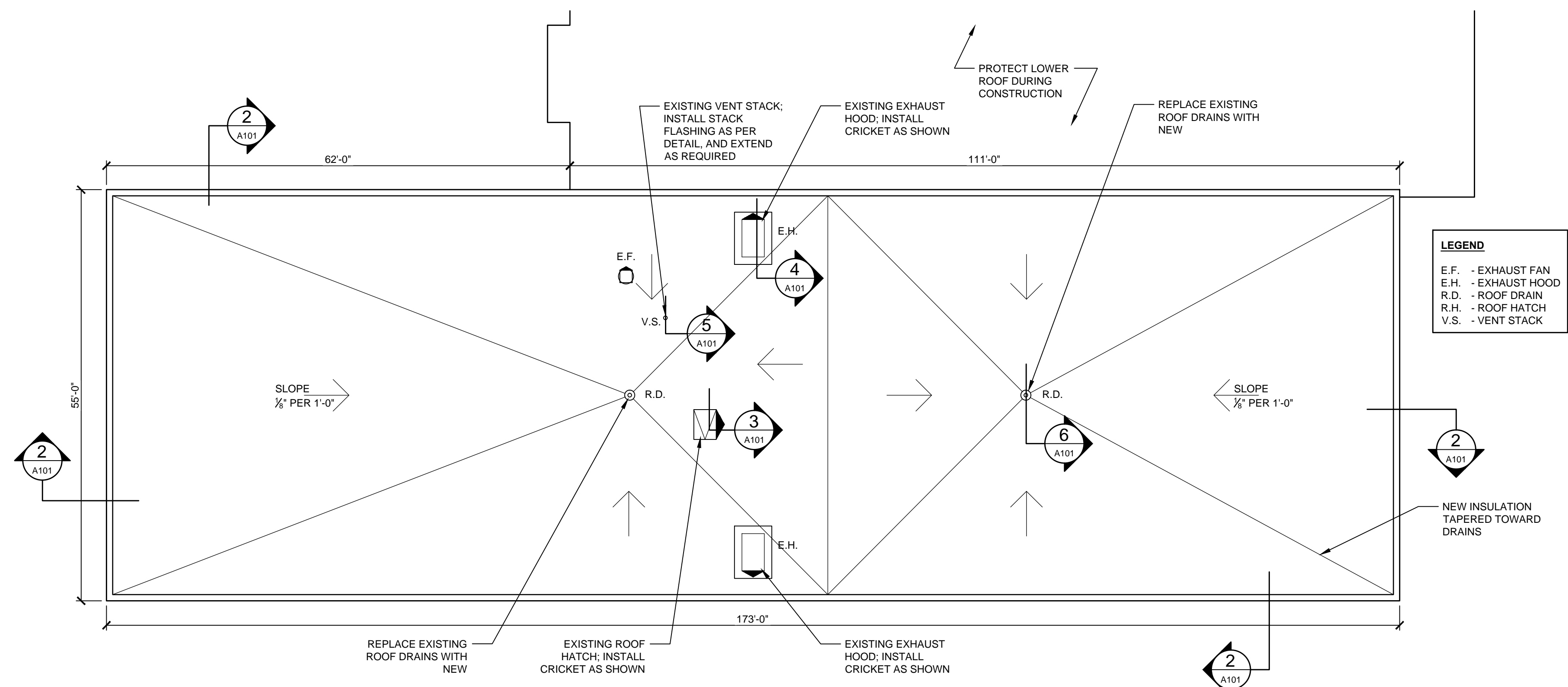
1 OVERALL ROOF PLAN A-101 3/32"-1'-0"
