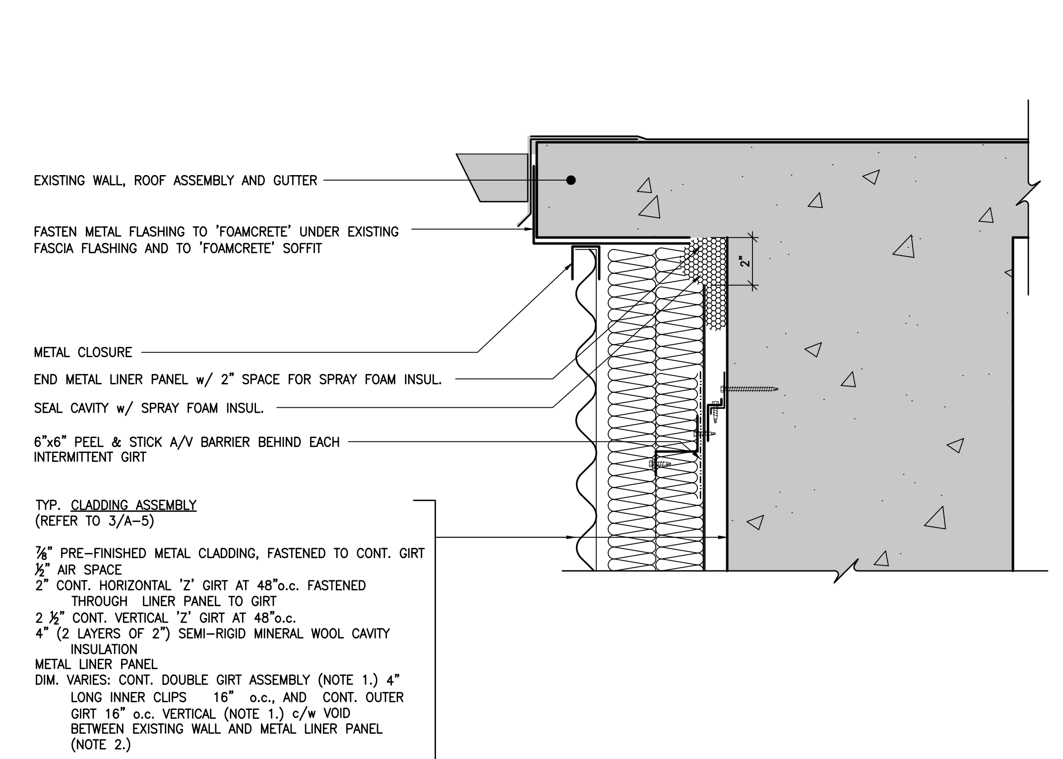
5 SECTION DETAIL - CLADDING AT ROOF EDGE 0 1" 2" 4" 8"
