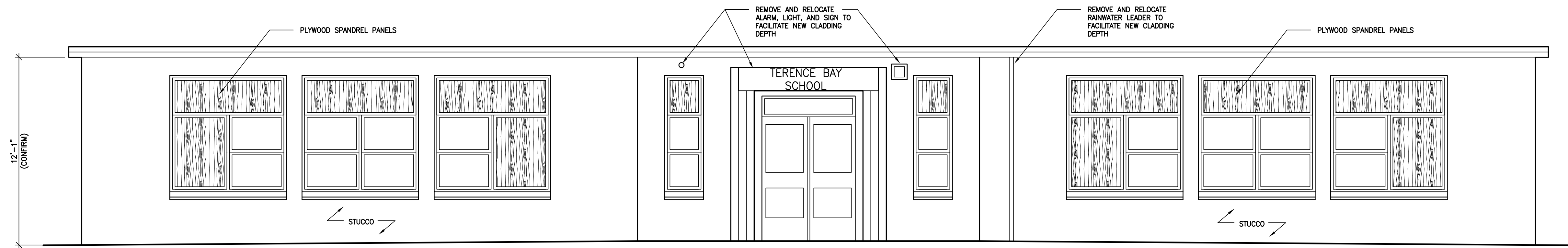
1 FRONT ELEVATION – EXISTING CONDITIONS
