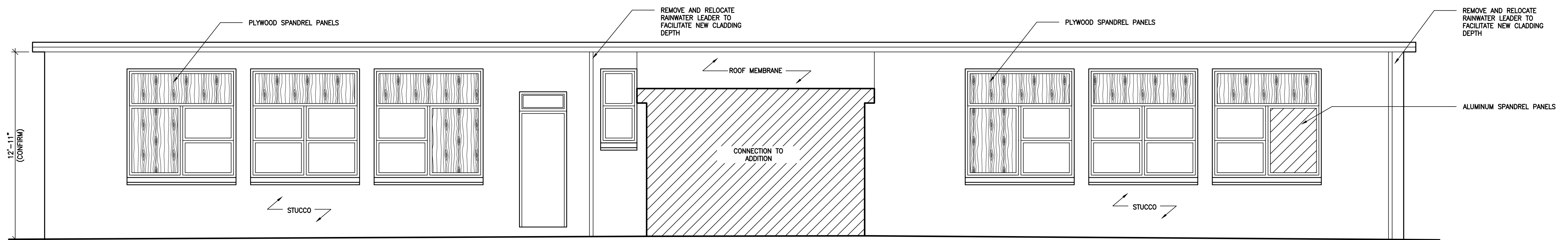
2 REAR ELEVATION – EXISTING CONDITIONS
