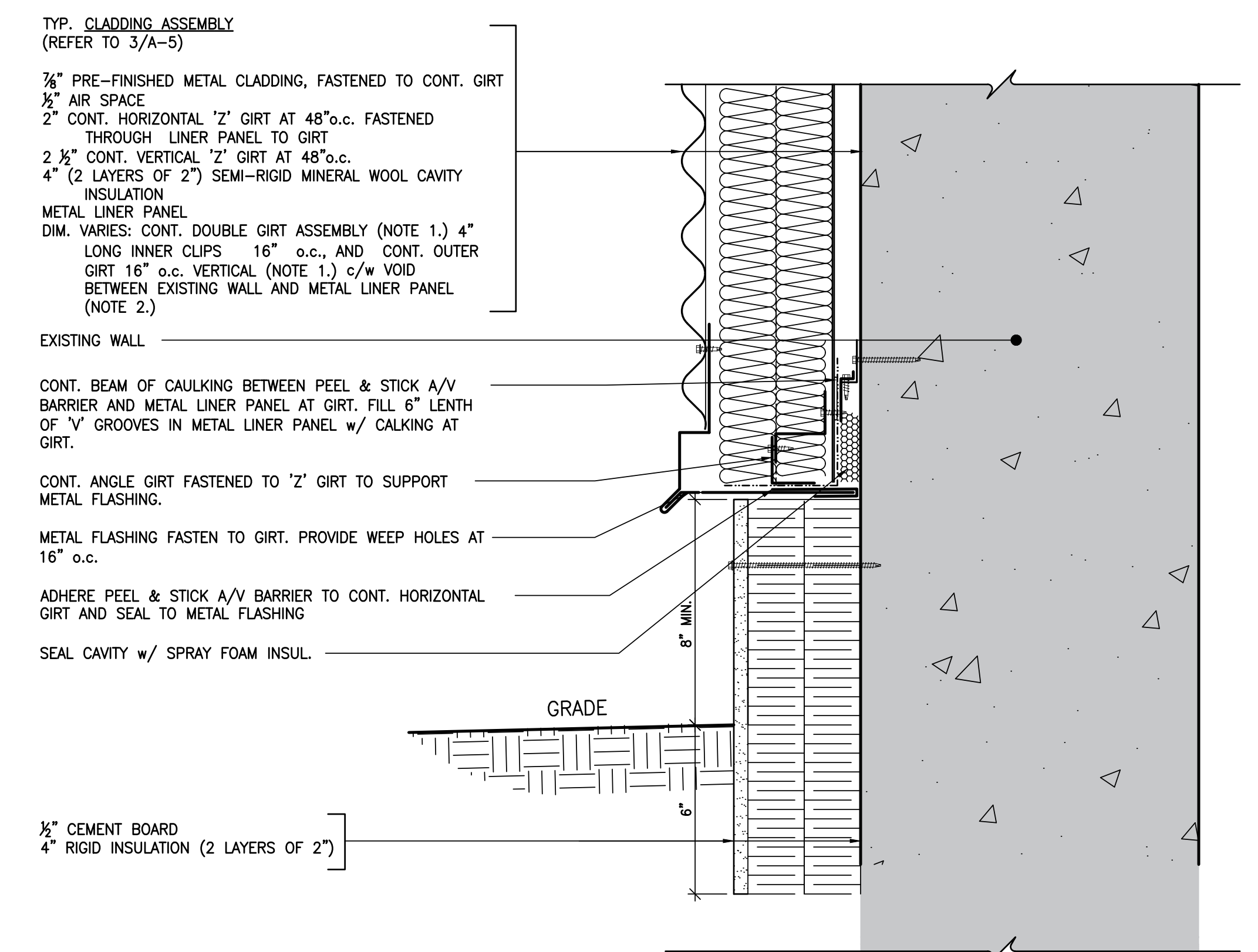
6 SECTION DETAIL - CLADDING AT GRADE 0 1" 2" 4" 8"
