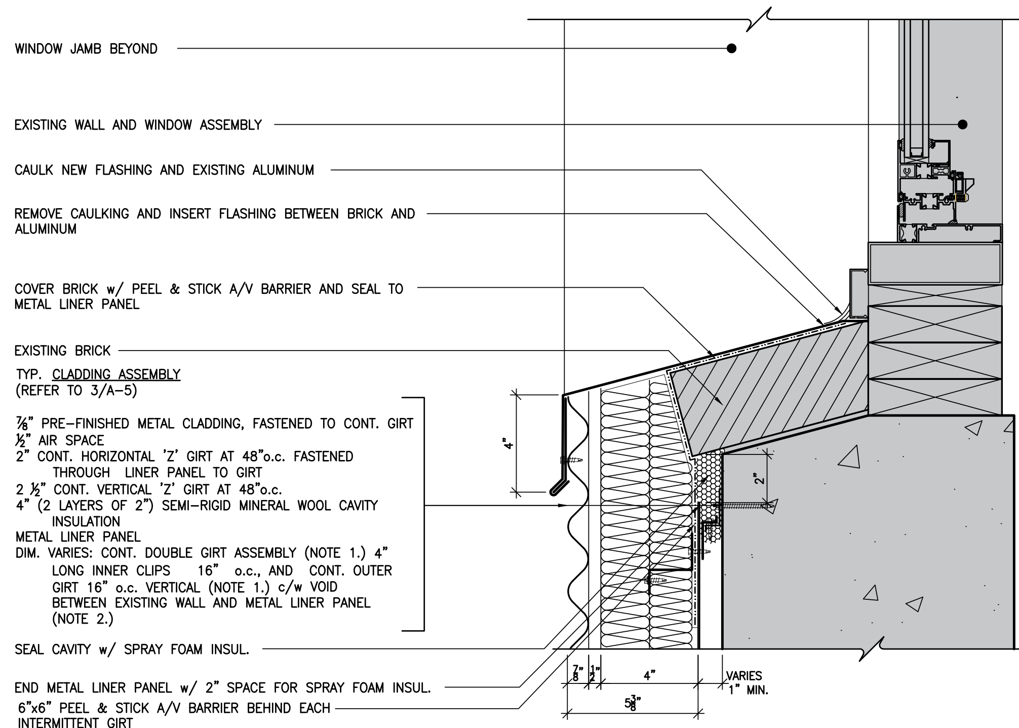
2 SECTION DETAIL - CLADDING AT WINDOW SILL 0 1" 2" 4" 8"
