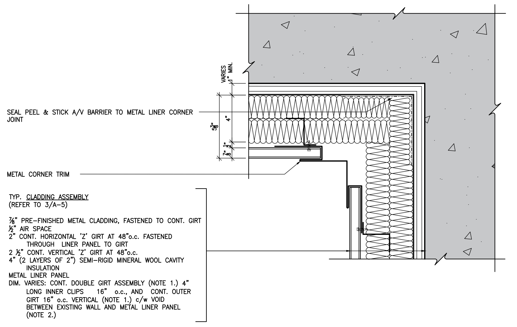
5 PLAN DETAIL - CLADDING AT FRONT ENTRANCE 0 1" 2" 4" 8"
