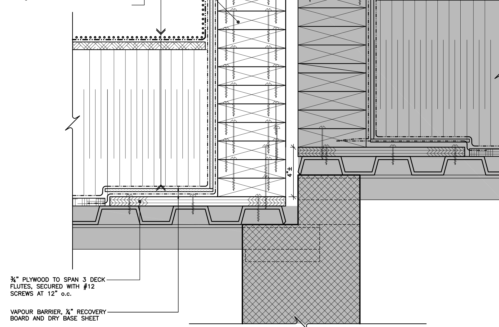
4 SECTION DETAIL ROOF DIVIDER AT GYM SCALE: 3" = 1'-0"
