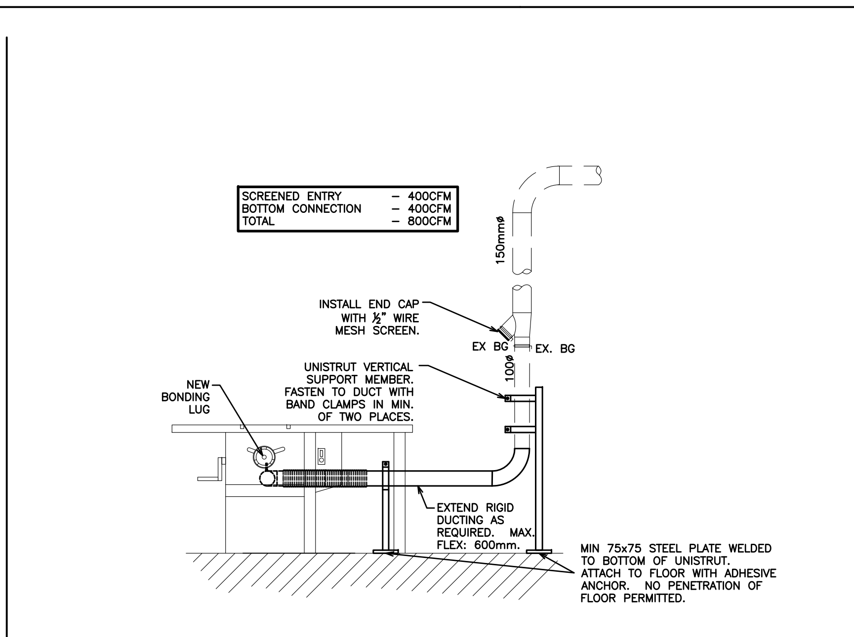
M-101 REVISED SAWSTOP TABLE SAW DETAIL
