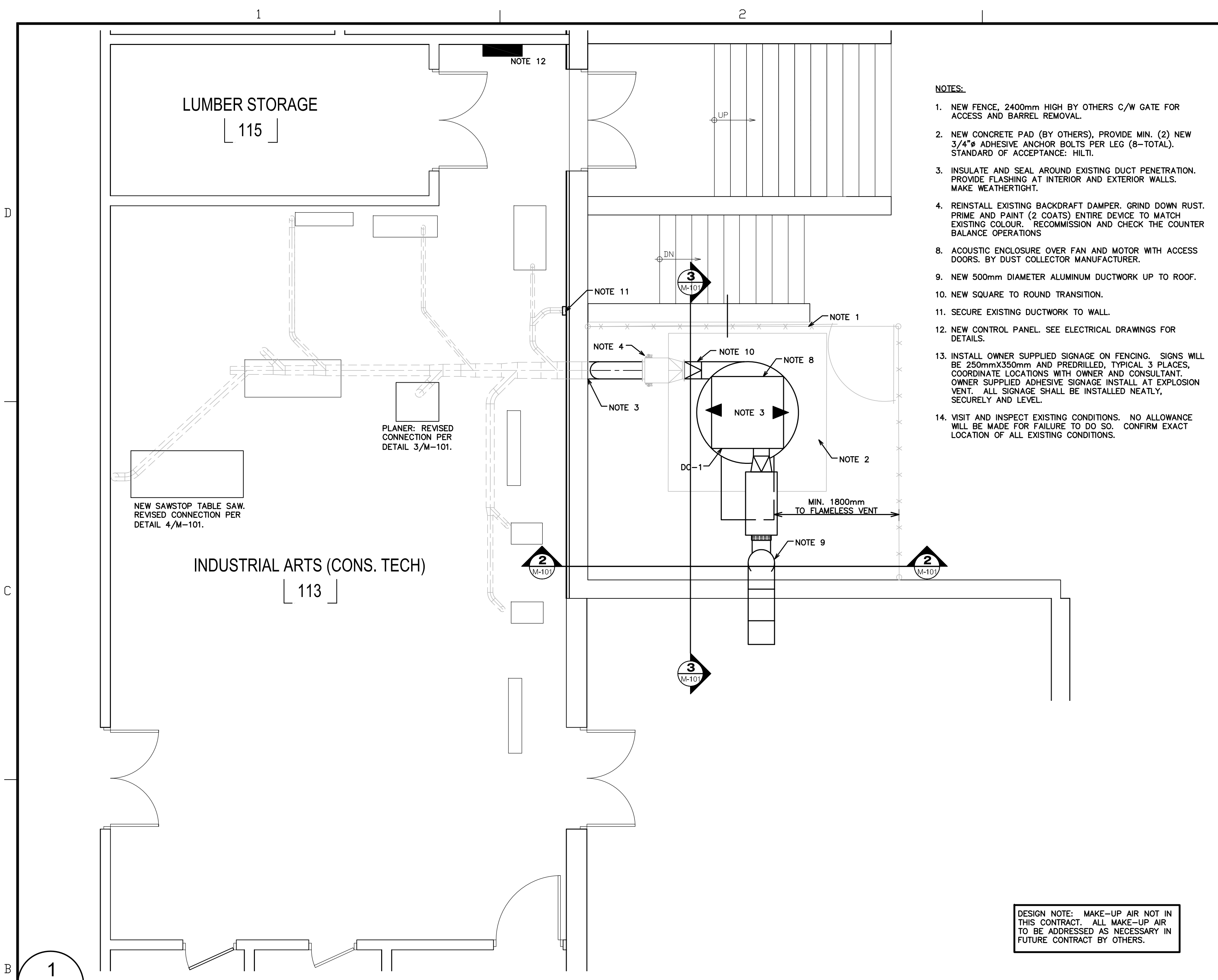
M-101 DUST COLLECTOR DUCTWORK PLAN
