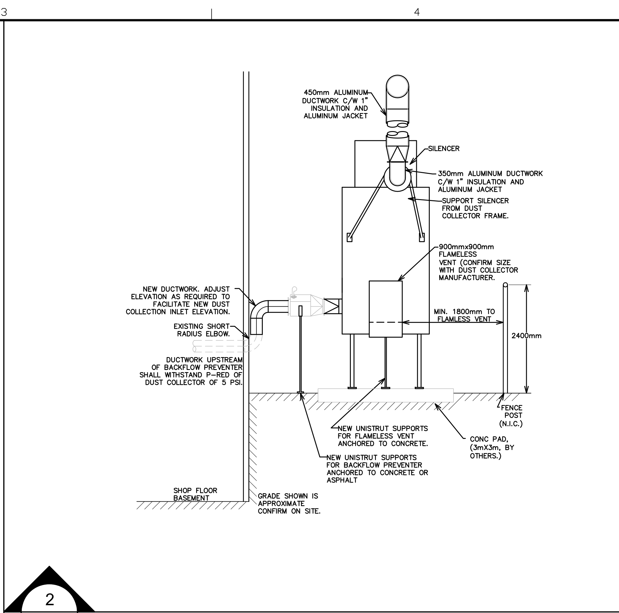
M-101 DUST COLLECTOR SOUTH ELEVATION
