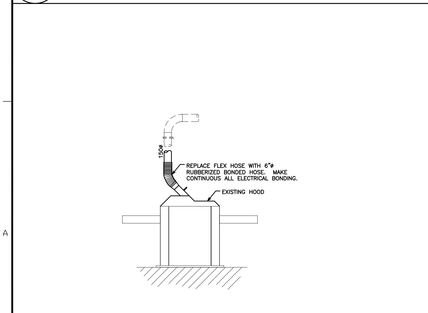
M-101 REVISED PLANER DETAIL
