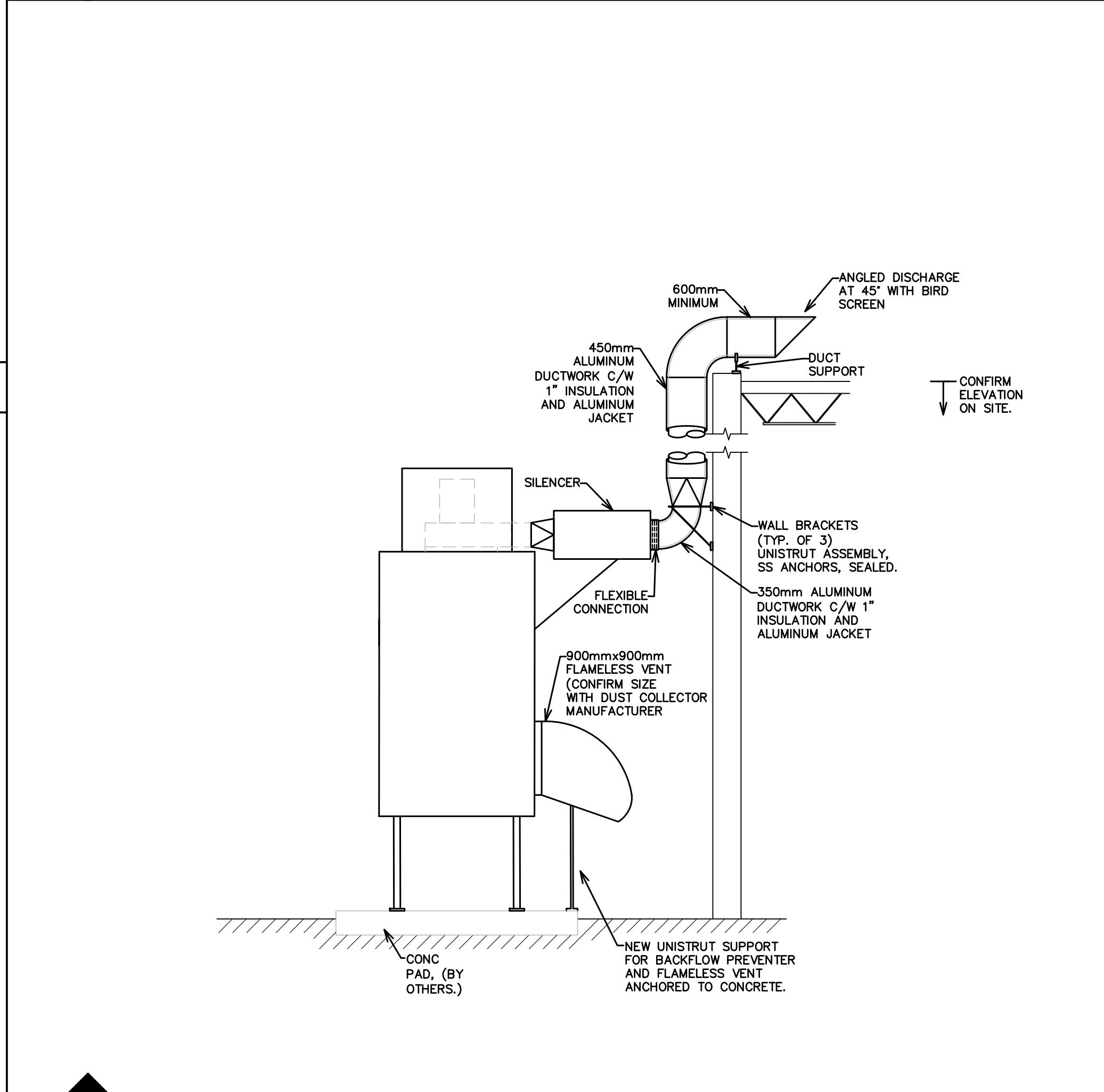
M-101 DUST COLLECTOR WEST ELEVATION
