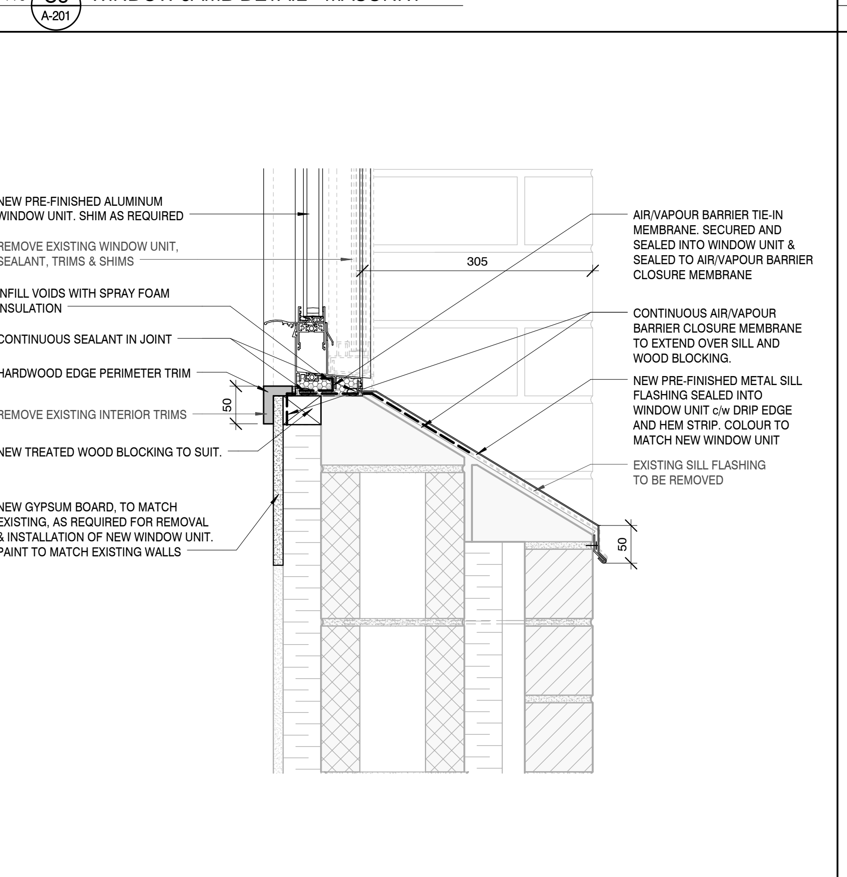
1:5 D3 WINDOW SILL DETAIL - MASONRY
