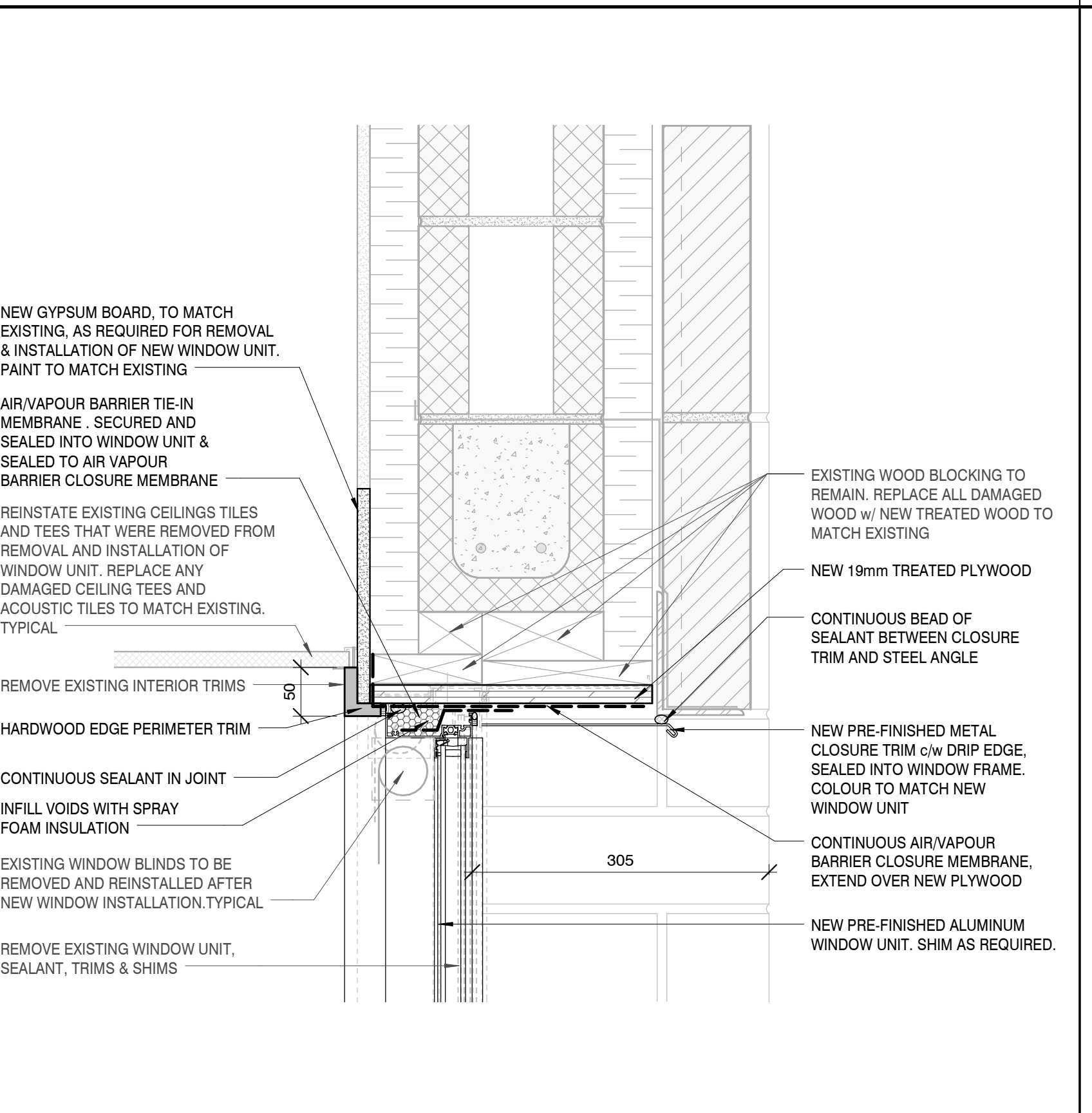
1:5 B3 WINDOW HEAD DETAIL - MASONRY
