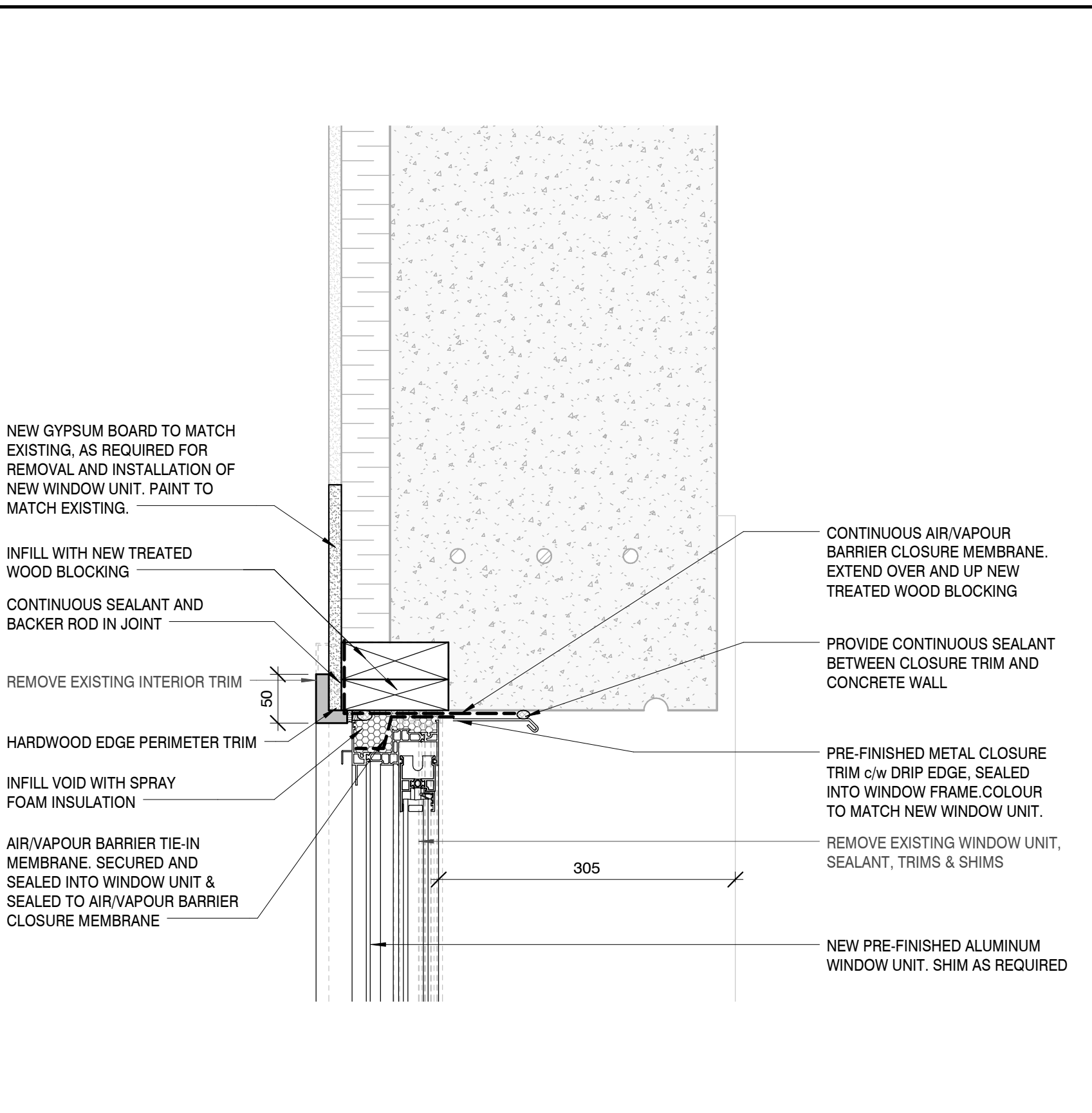
1:5 B4 WINDOW HEAD DETAIL - CONCRETE
