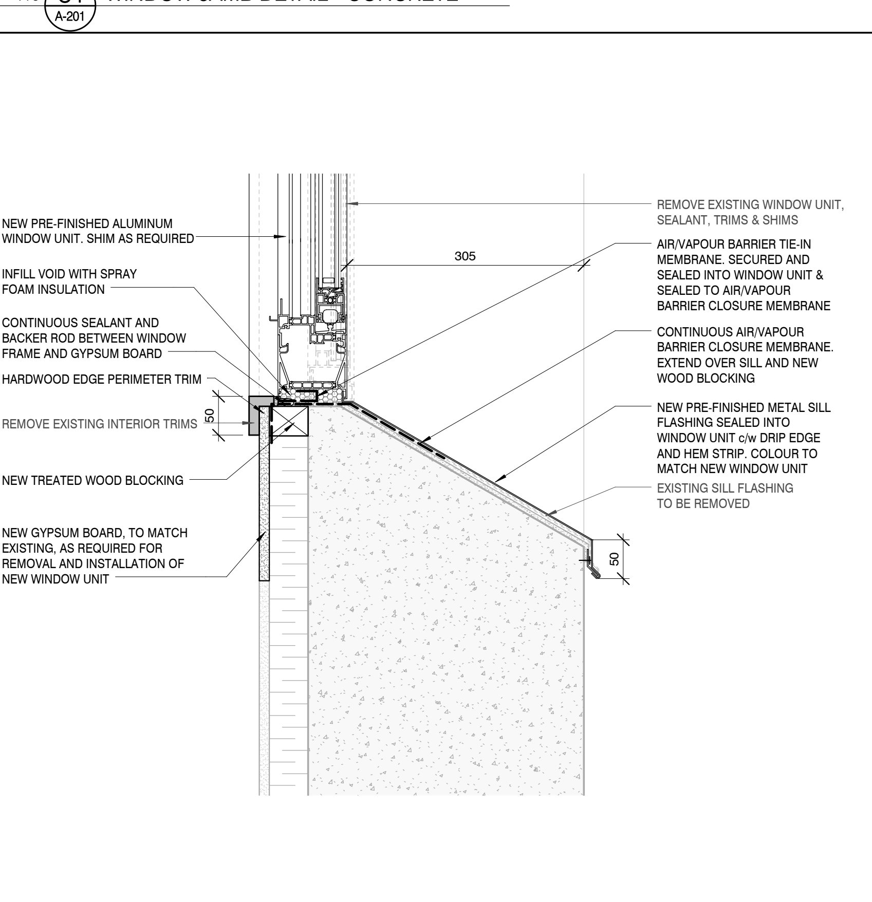
1:5 D4 WINDOW SILL DETAIL - CONCRETE
