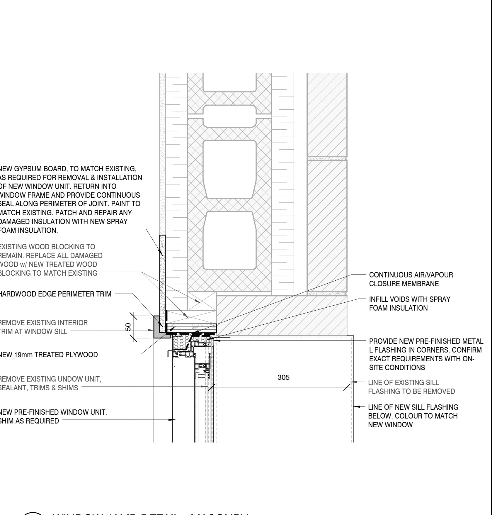
1:5 C3 WINDOW JAMB DETAIL - MASONRY
