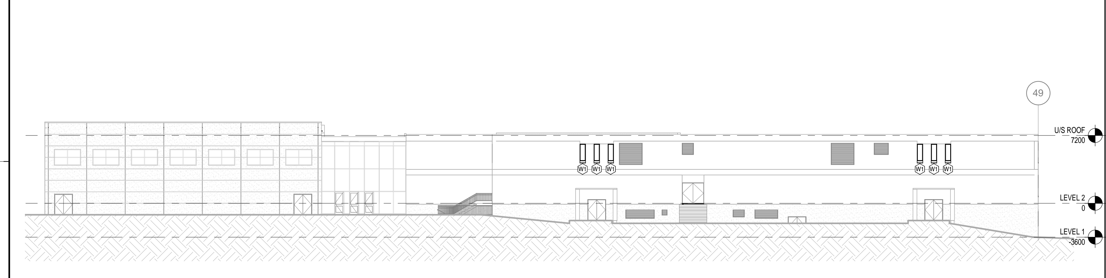
1:250 C1 NORTH ELEVATION
