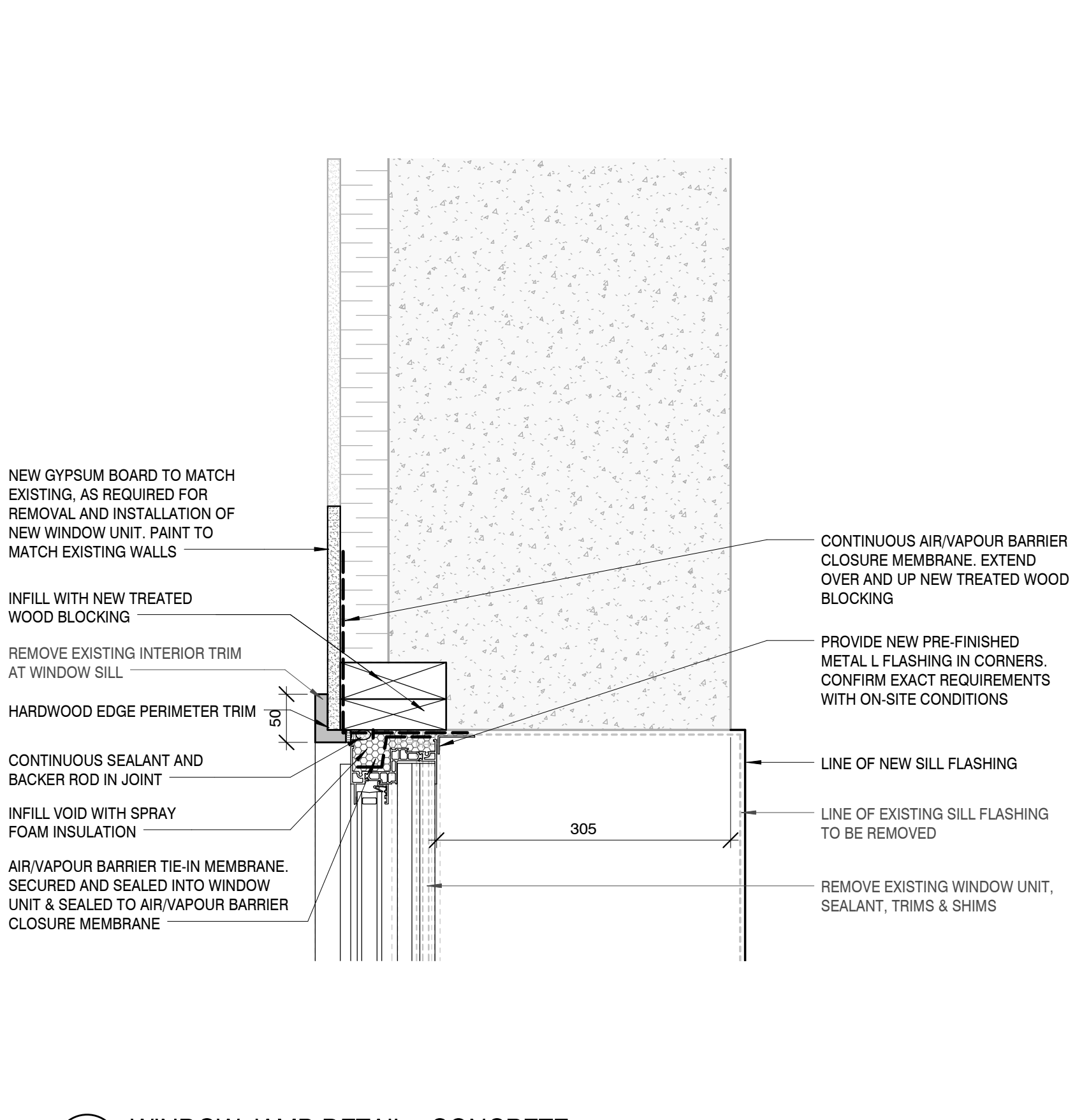
1:5 C4 WINDOW JAMB DETAIL - CONCRETE
