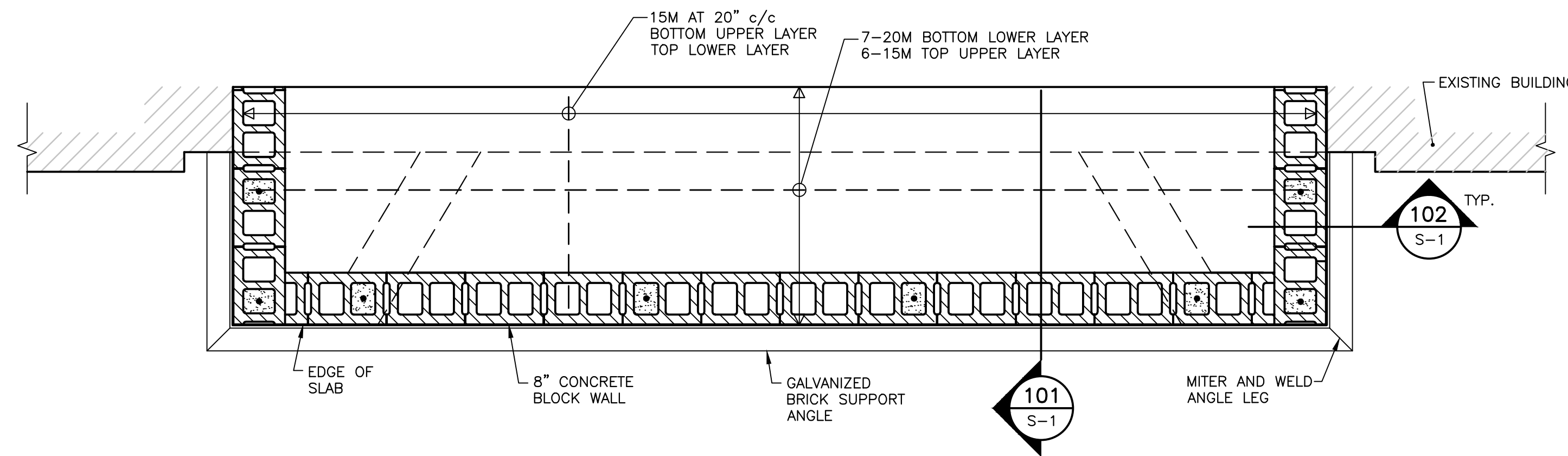
ROOF SLAB PLAN SCALE: 3/4"=1'-0"
