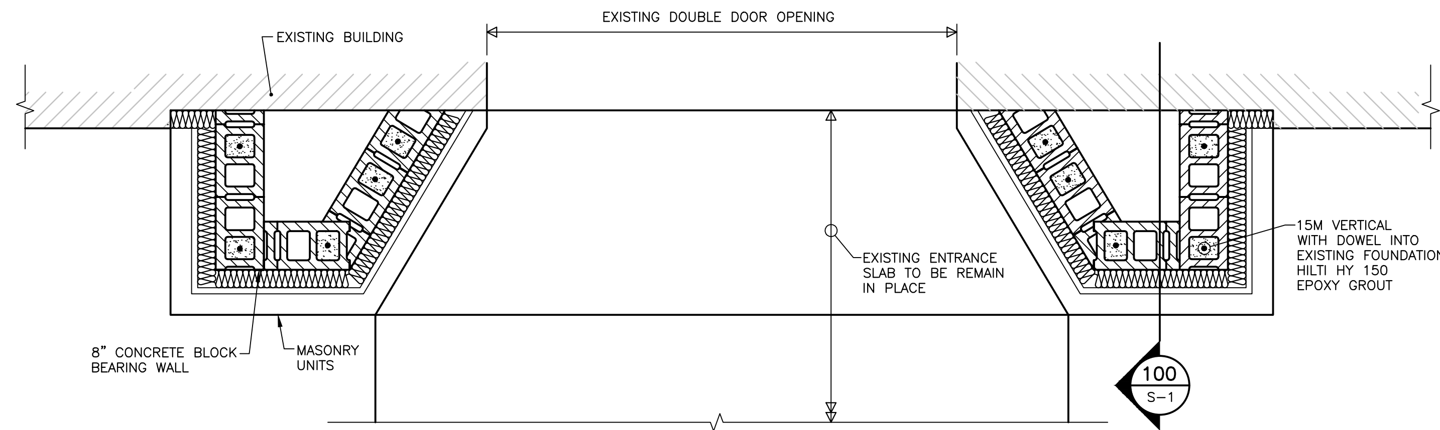
FOUNDATION PLAN SCALE: 3/4"=1'-0"
