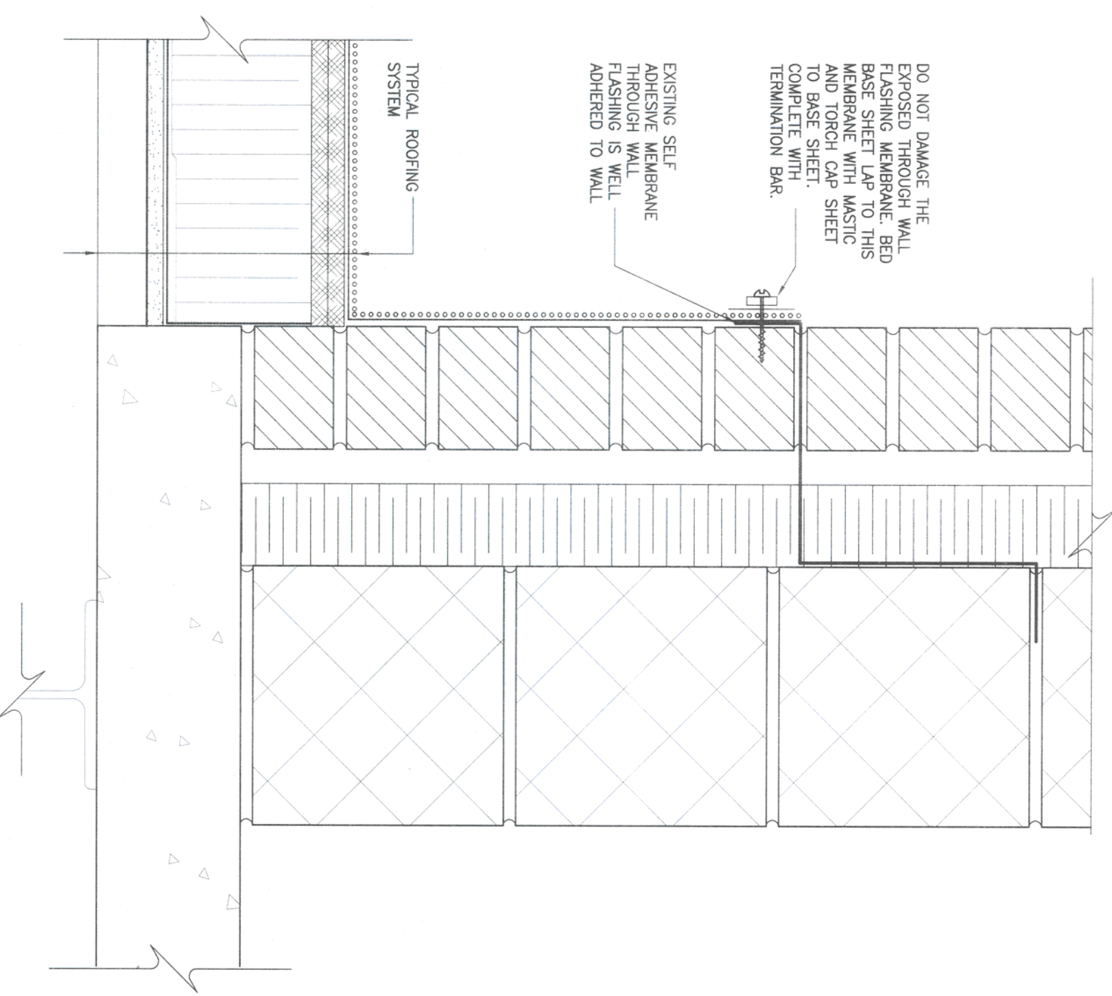
1 ROOF TO PENTHOUSE WALL
