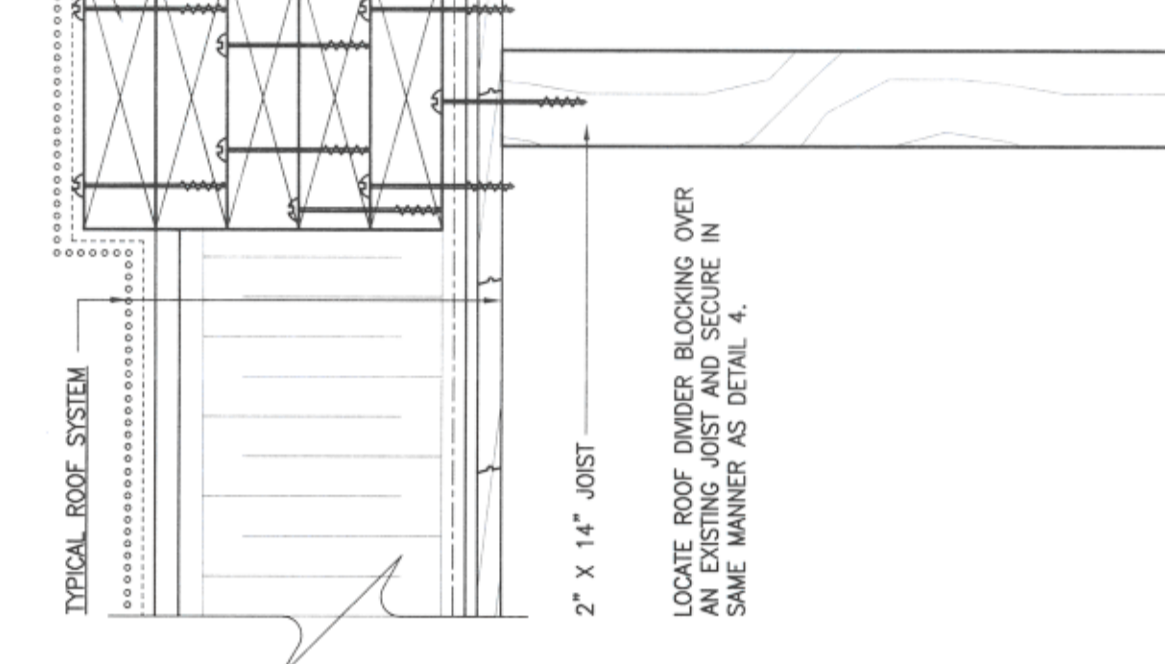
5 ROOF DIVIDER
