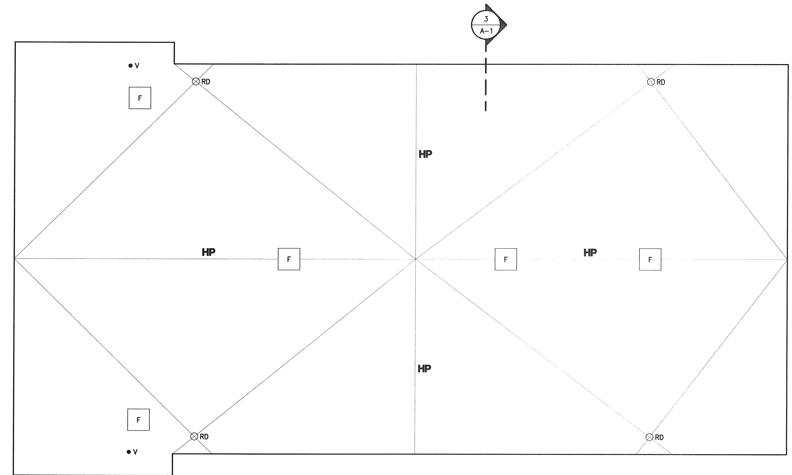
2 GYM ROOF PLAN 0 2 4 8 16 FEET
